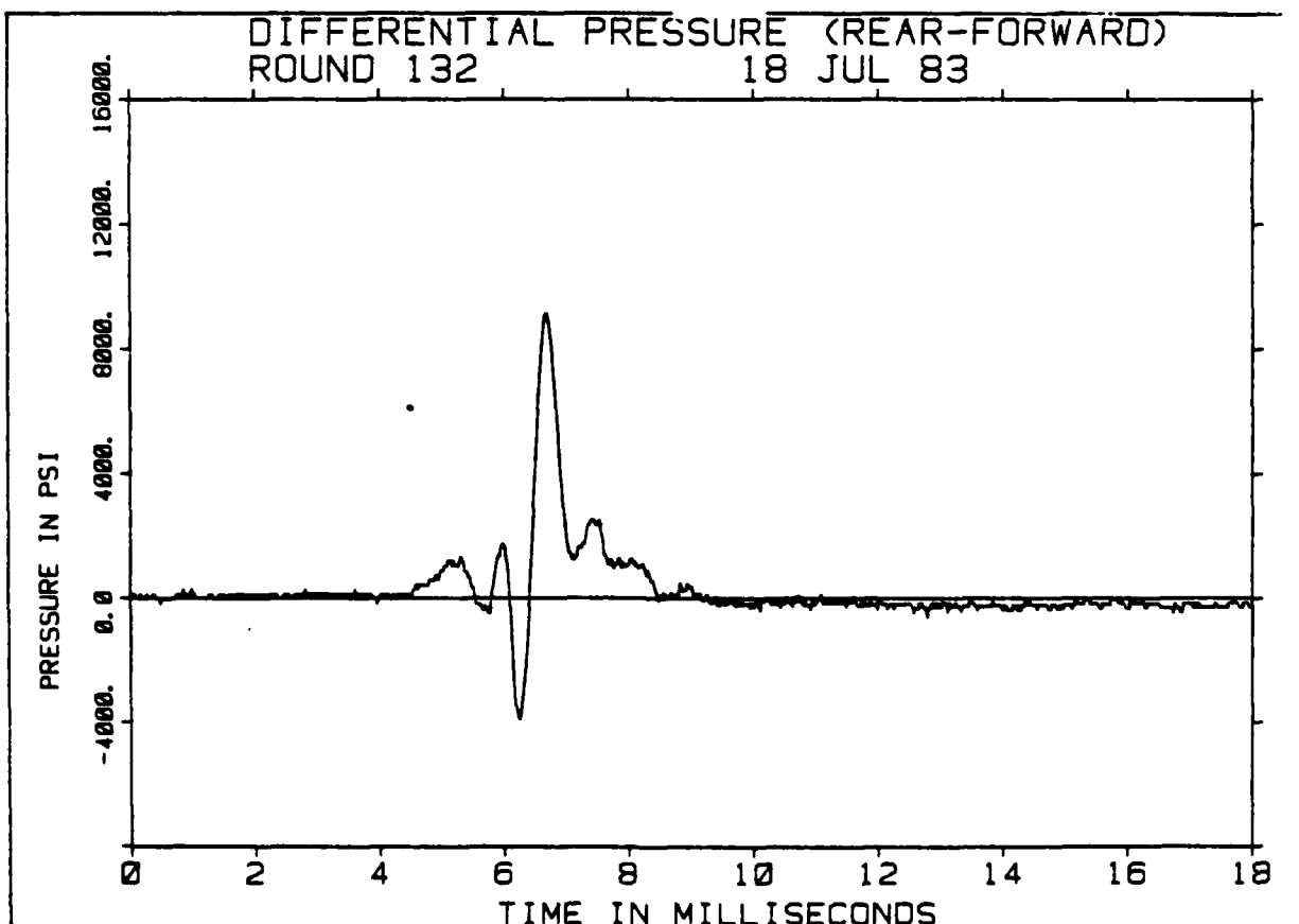
Figure 1.1-1. Example of a good differential pressure measurement.
