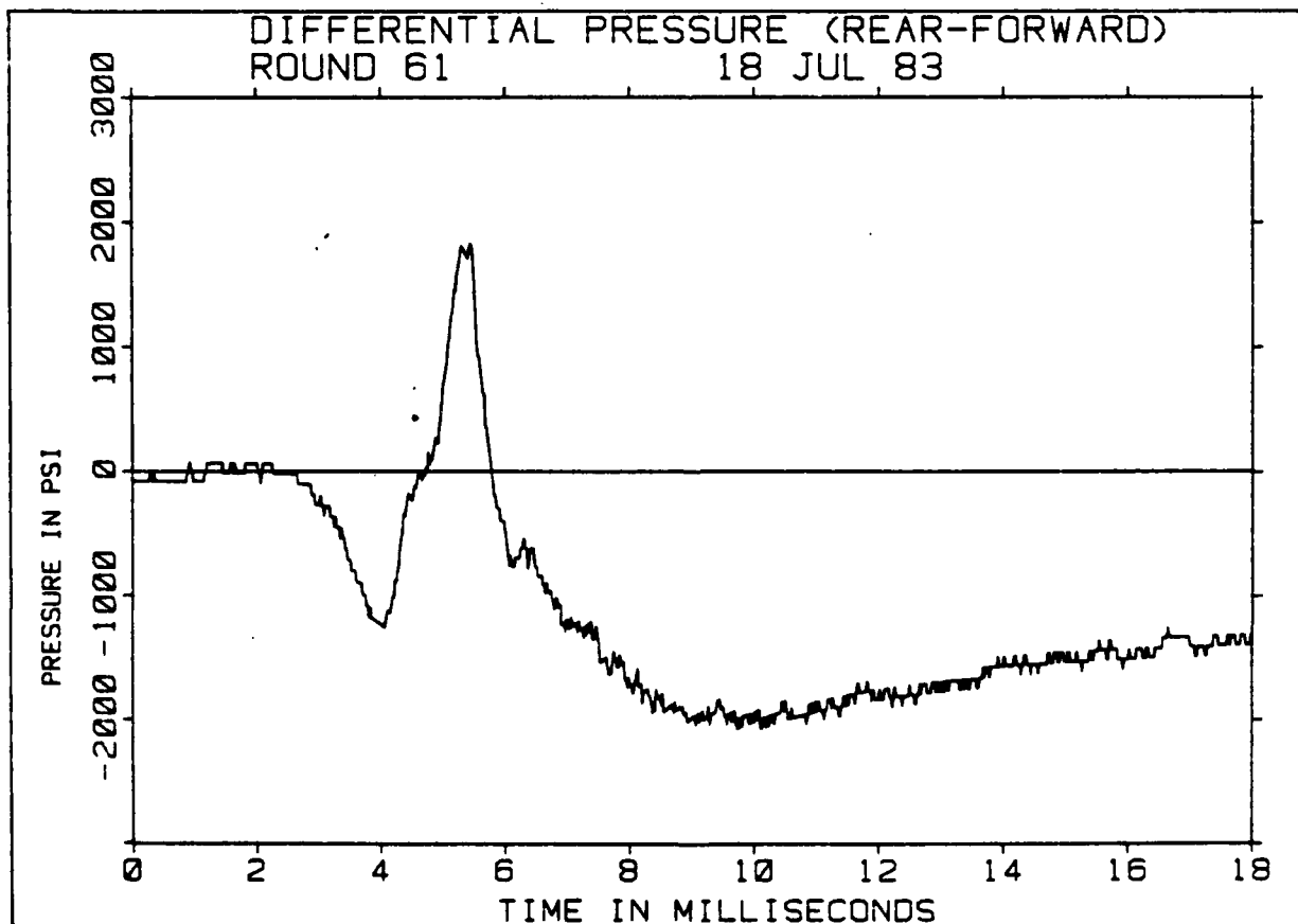
Figure 1.1-2. Example of a poor differential pressure measurement.
