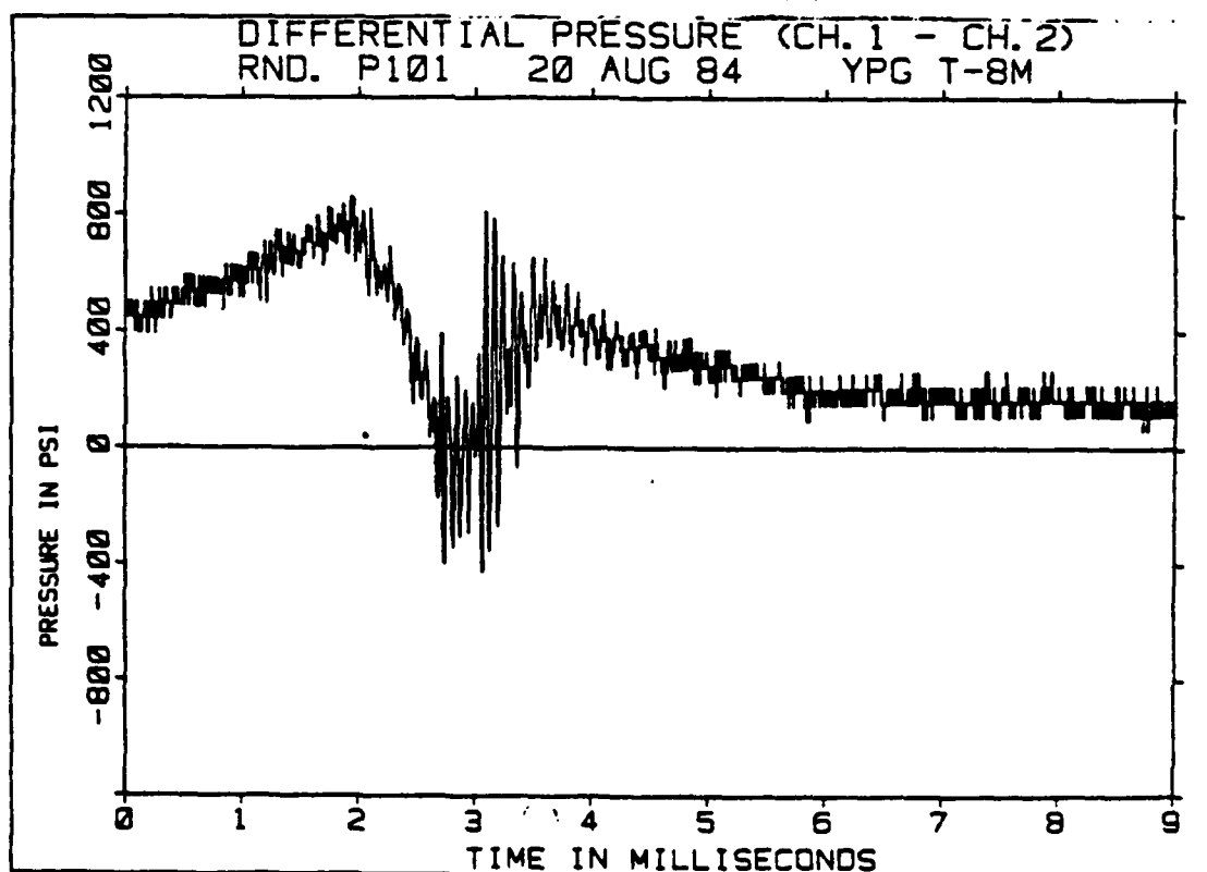
Figure 2.13-4. Pressure measurement from PCRL pressure generator using T-8M transducers.
