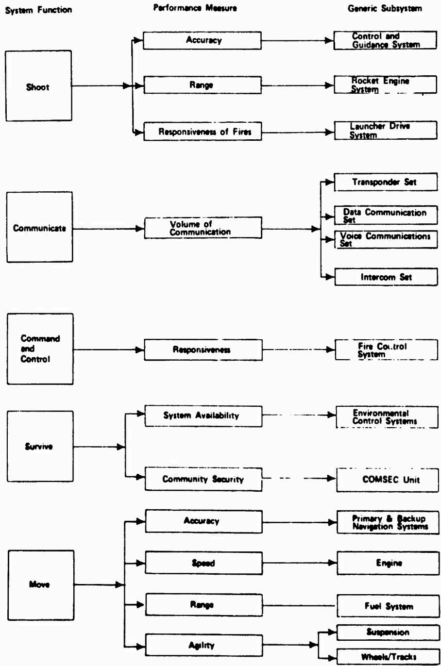
Figure 1.3-2. Functional allocation.
