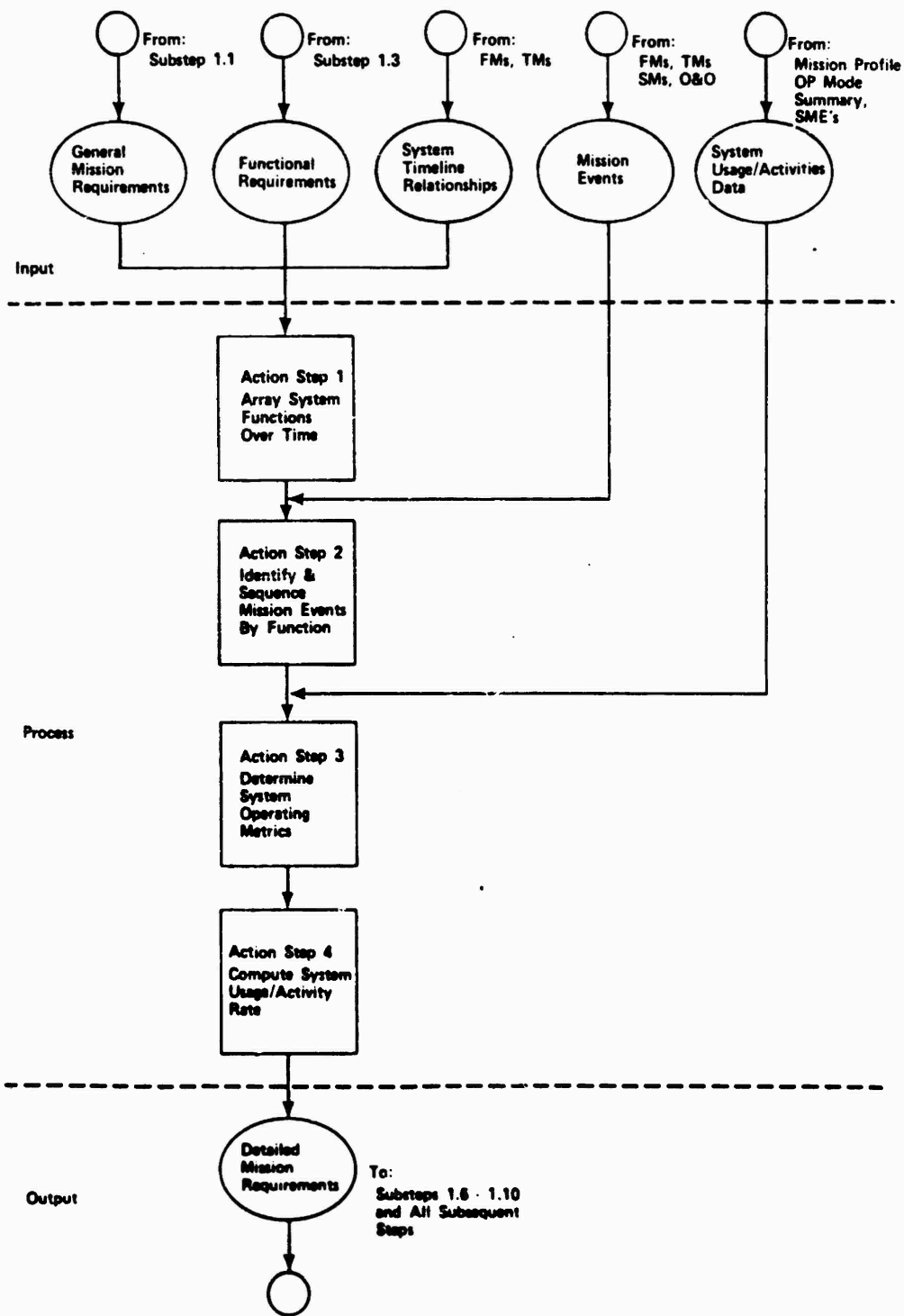
Figure 1.2-1. Logic flow for Detailed Mission Requirements.
