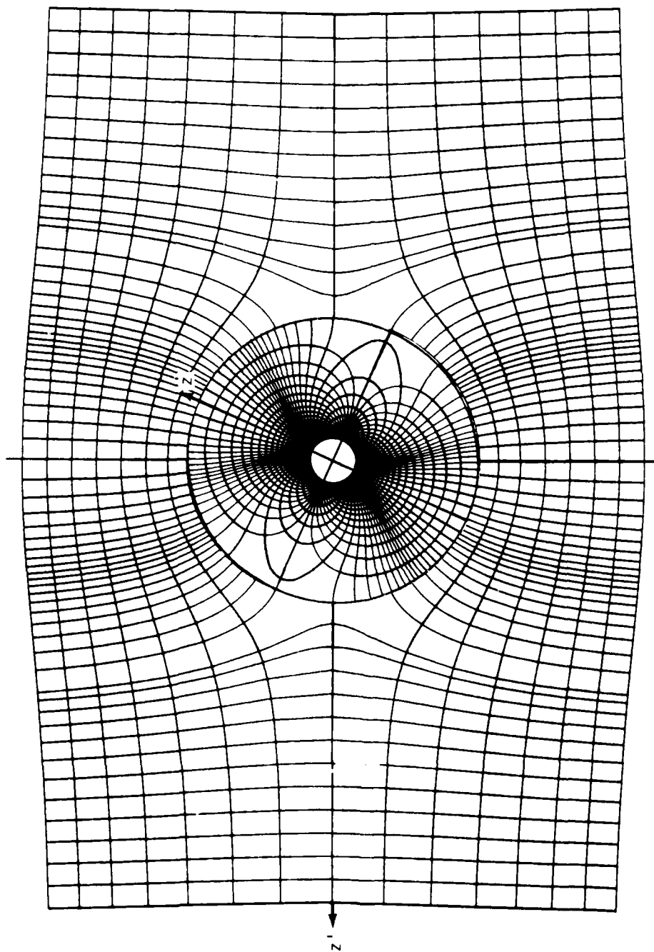
Figure 3c. An example of how Figures 3a and 3b might be rejoined to generate a complete mesh. The spherical nature of the interface at r=k^{1/3} allows the z and z' axes to be oriented arbitrarily with respect to one another.
