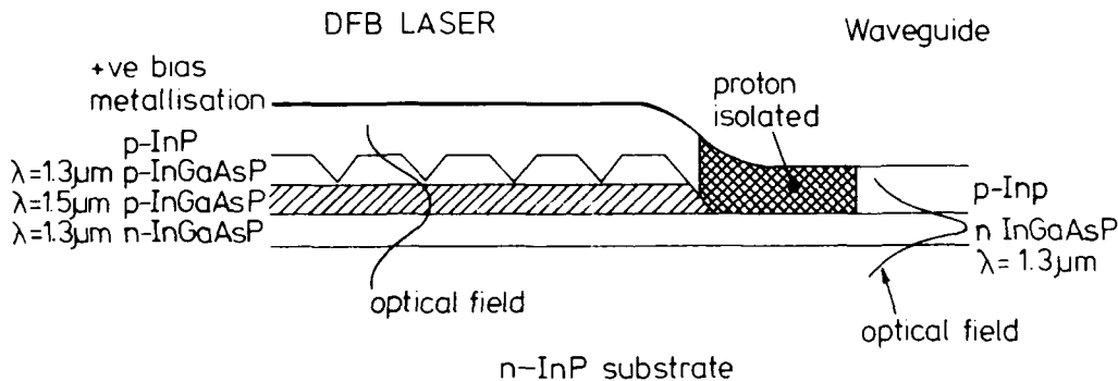
FIG 4 A scheme for integrating a DFB laser with a waveguide
