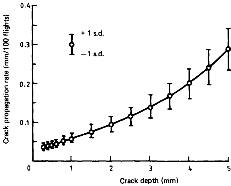
(a) Crack propagation rates
