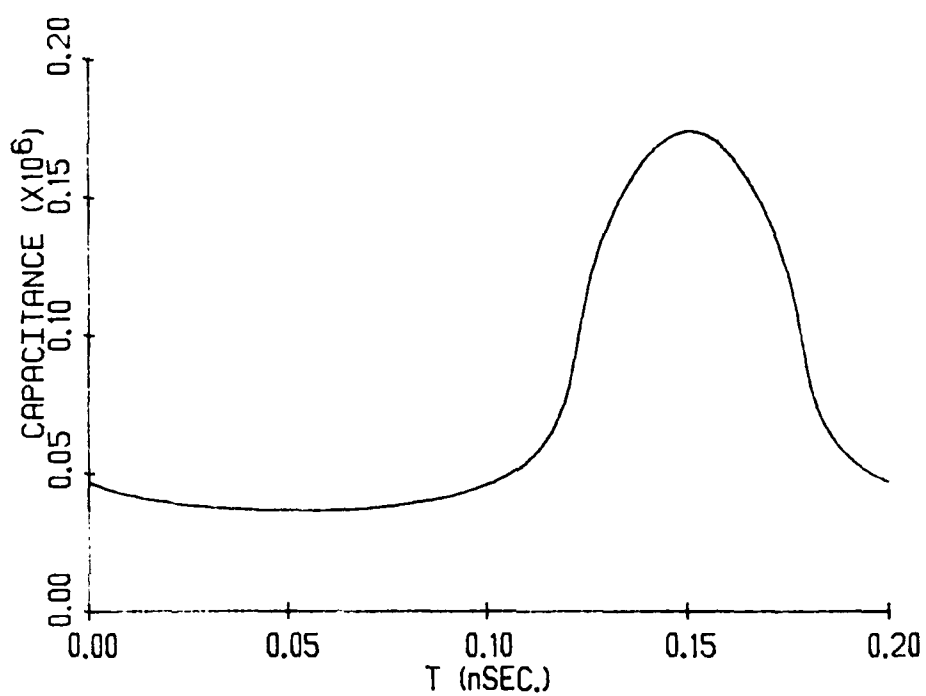
FIG. 19 CAPACITANCE/cm 2 FOR THE PROFILE IN FIG. 16 SUBJECTED TO THE VOLTAGE OF Fig. 18.
