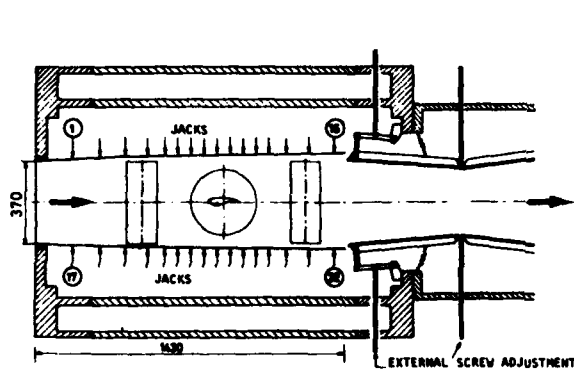
FIGURE 5 TUNNEL CHARACTERISTICS OF T2
