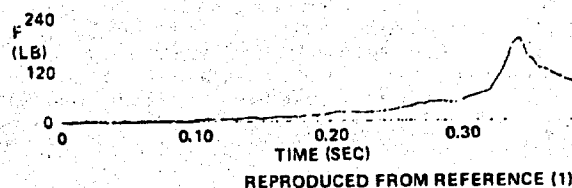
FIG. 3 TYPICAL FORCE-TIME CURVE FOR A 10% EXTENDED SKIRT PARACHUTE UNDER INFINITE MASS CONDITIONS.
