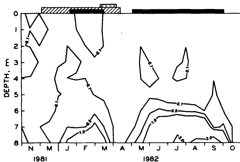
Figure 49. Vertical changes in total manganese concentration for the two study periods. Periods of anoxia (solid bar), ice cover (hatched bar), and spring runoff (cross-hatched bar) are indicated.
