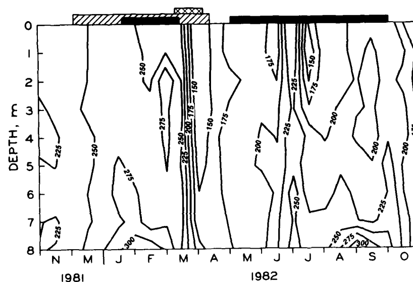
Figure 34. Vertical changes in total solids concentration for the two study periods. Periods of anoxia (solid bar), ice cover (hatched bar), and spring runoff (cross-hatched bar) are indicated.
