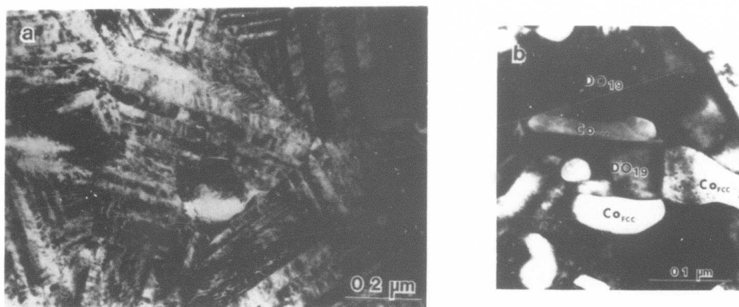
Fig. 2. Co-34 Sn alloy. (a) Martensitically transformed grains near the wheel side; (b) interlocked structure of \alpha\text{-Co} and \text{Co}_3\text{Sn} at the ribbon center.
