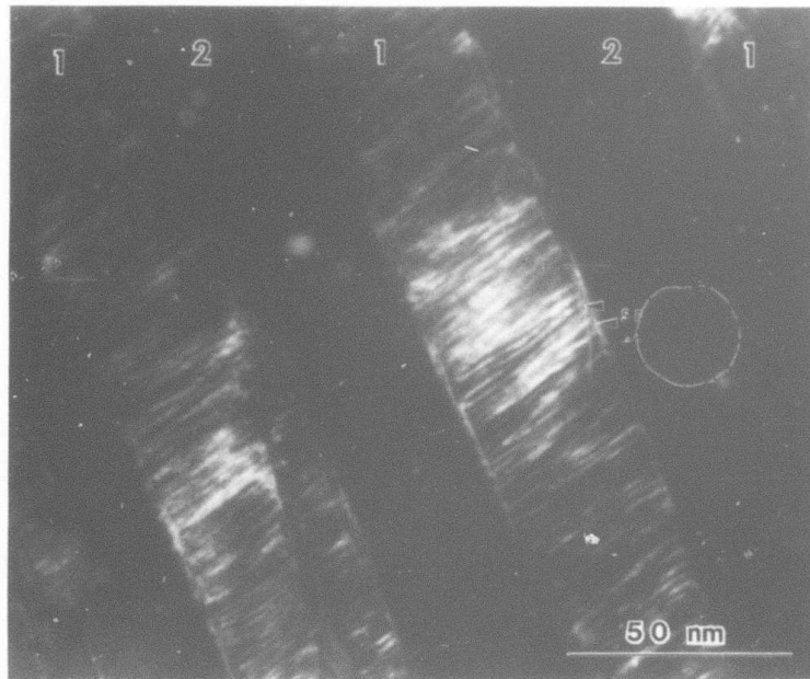
Figure 4: Dark field image of the 2H martensite. Twin variant 1 shows high density stacking faults.
