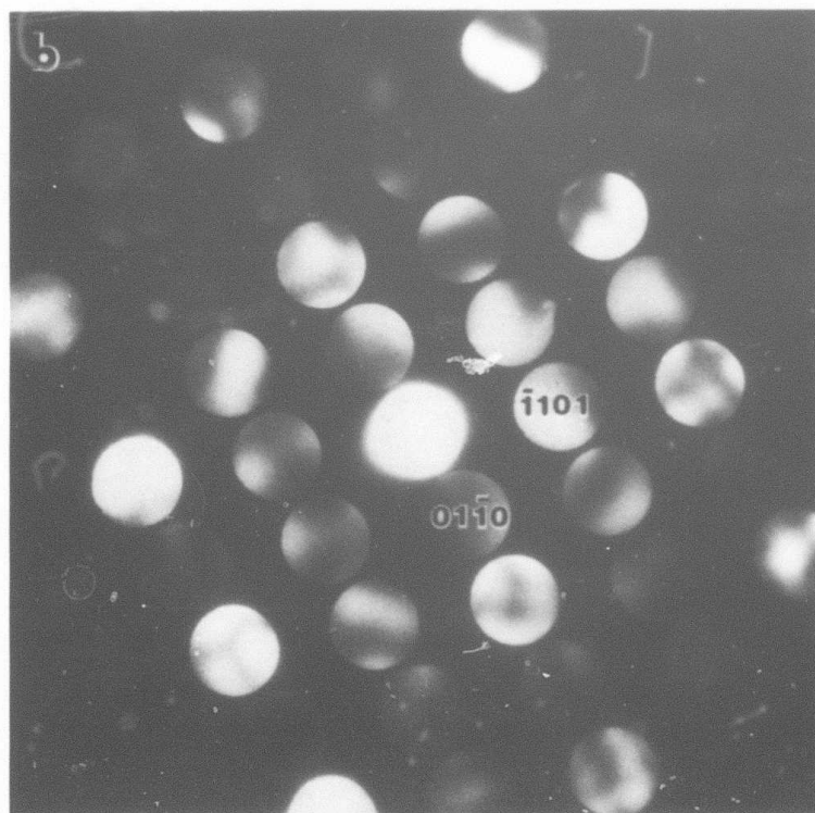
Figure 8: Electron diffraction patterns taken from intermetallic phase yielding hexagonal \text{DO}_{19} structure: (a) zone axis 2\bar{1}\bar{1}0 , (b) zone axis 2\bar{1}\bar{1}3 .
