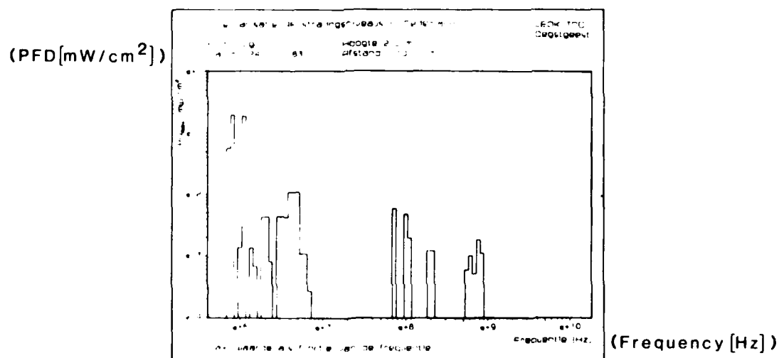
Figure 3. Plot of maximum PFD versus frequency of a subset of transmitters.
