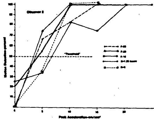
Fig. 2. Thresholds for detection of linear oscillation for Astronaut 2. The R+O data were obtained 75 minutes after landing.
