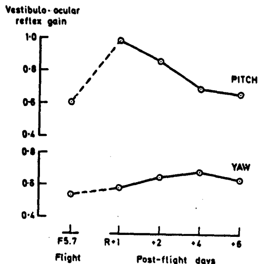
Fig 3. Vestibulo-ocular reflex gain during voluntary head oscillation at 1 Hz with eyes closed. Mean values for astronauts C & D.
