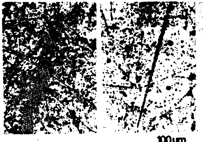
Fig. 2: Track of the heaviest ion ever detected in the Biostack experiments, on the left side penetrating through a 300 \mu\text{m} thick K5 emulsion, on the right side its stopping end in a 300 \mu\text{m} thick neighbouring K2 emulsion
