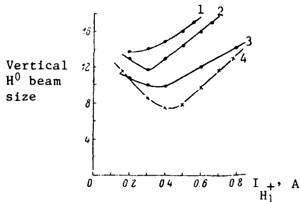
Fig. 20--Vertical neutral hydrogen beam size as a function of H_1^+ beam current, with beam collector placed 2.2 m from ion source [104] 1--15 keV beam energy 2--20 keV 3--25 keV 4--25 keV, with reduced angular spread approaching Pierce geometry
