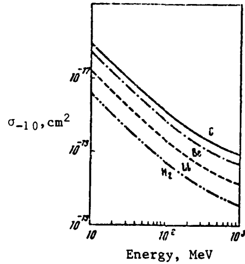
Fig. 37--Calculated electron loss cross sections ( \sigma_{-10} ) from H^- ions in H_2 and in Li, Be, and C atoms [97]
