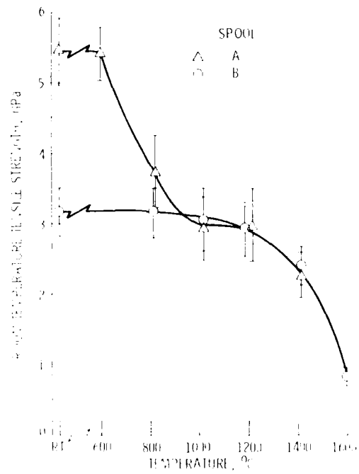
Figure 4. Tensile strength of carbon coated Saffil fibers after 15 min exposure to oxygen at indicated temperatures.
