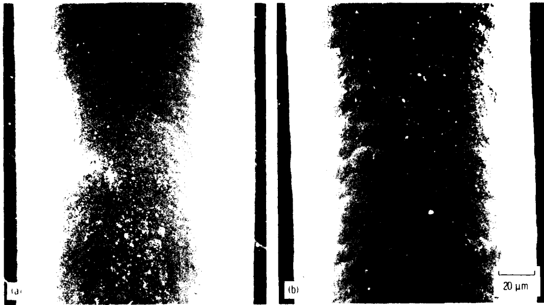
Figure 3. Photomicrographs showing surface microstructure on untreated, as-received carbon coated Saffil fibers, (a) Spool A; (b) Spool B.
