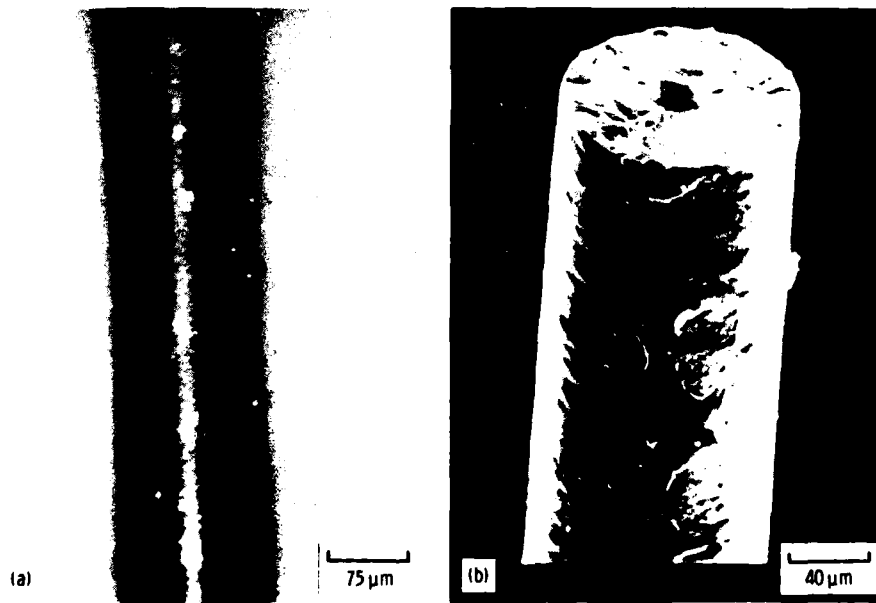
Figure 8. - (a) Photomicrograph of carbon coated SiC fiber heated at 1600 °C in air for 15 minutes showing bubbles and pits on the surface. (b) SEM photograph of a typical tensile fracture surface showing source of fracture.
