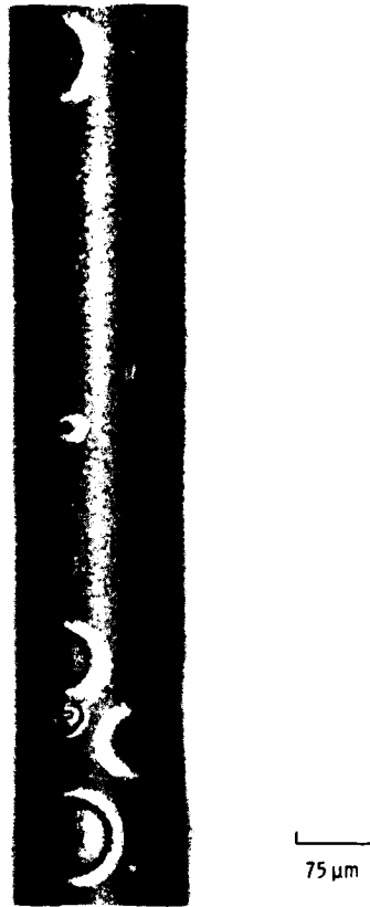
Figure 12. - Photomicrographs of SCS-6 fiber heated at 1200 °C in oxygen for 15 minutes showing pits and pinhole porosity on the surface.
