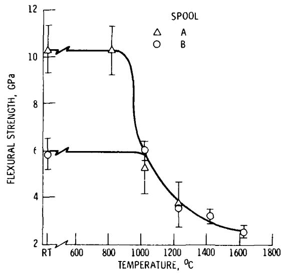
Figure 7. - Flexural strength of carbon coated SiC fibers at room temperature after 15-min exposure to vacuum at indicated temperatures.
