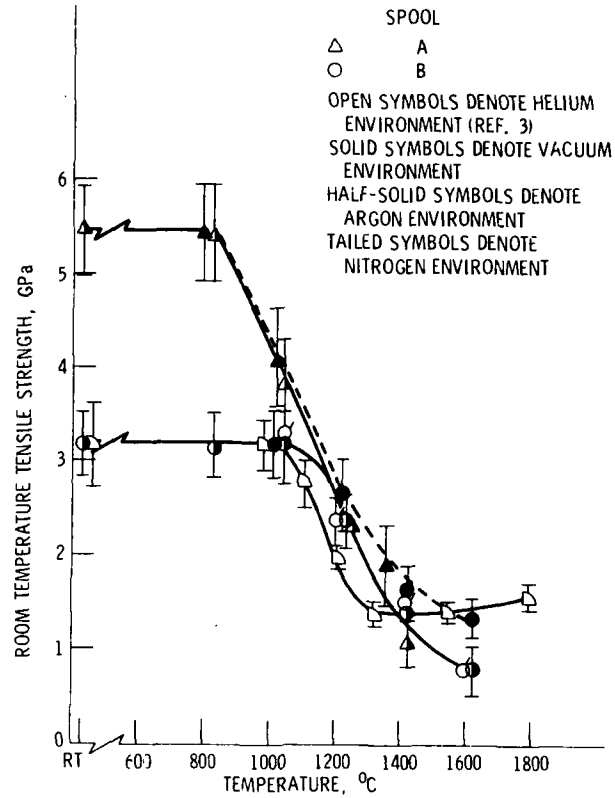
Figure 5. - Tensile strength of carbon coated SiC fibers after 15-minute exposure to various environments at indicated temperatures.
