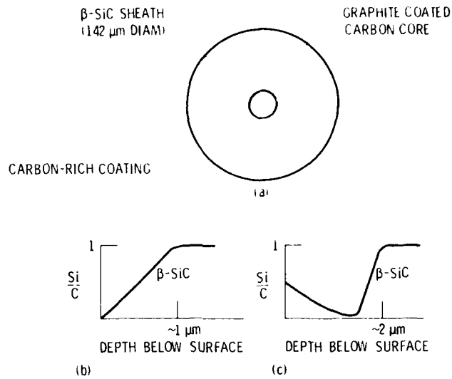
Figure 1. - (a) Schematic diagram of cross-section of coated AVCO (CVD) SiC fiber. (b) and (c) The composition of carbon-rich coating near the surface of carbon coated SiC fiber and SiC/C coated SiC fiber (SCS-6).
