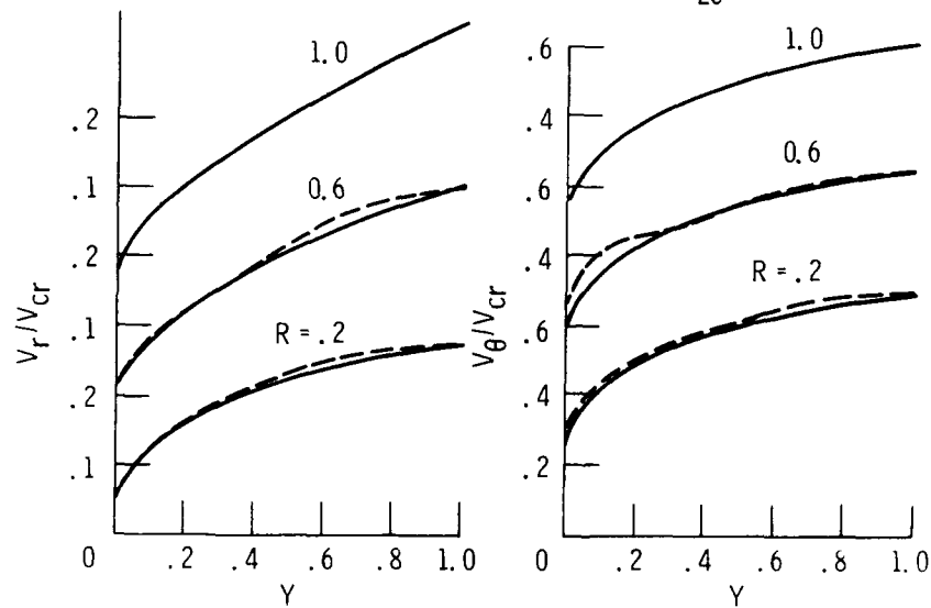
(e) Case V: Fully developed flow; \alpha_{2e} = 70^\circ .
