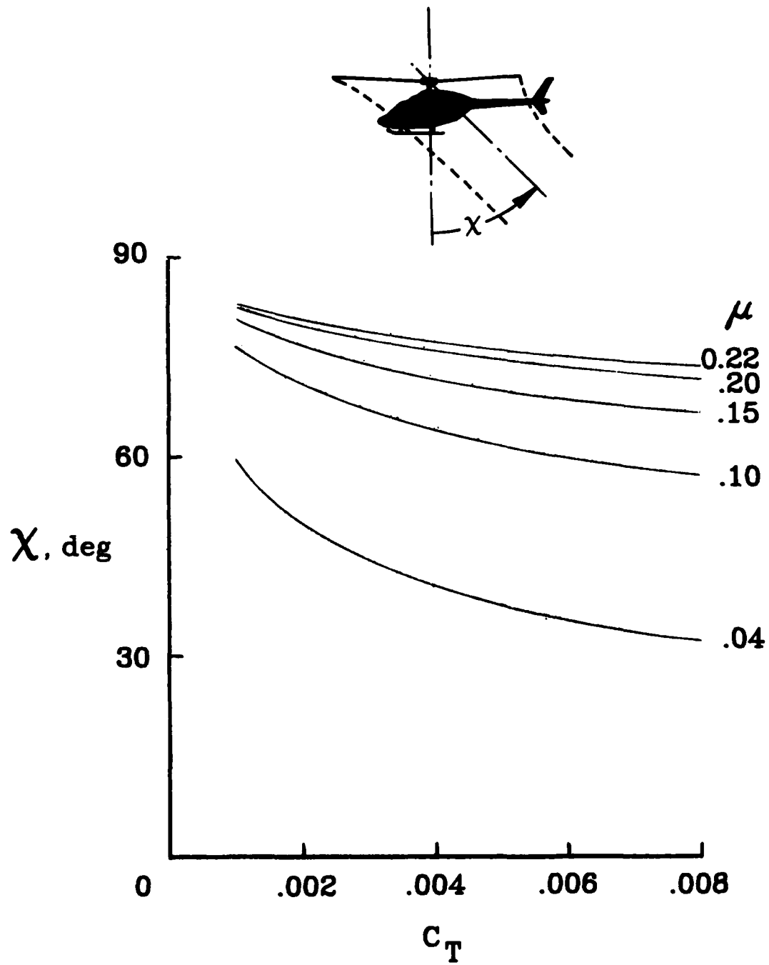
Figure 17. Effect of thrust coefficient on wake skew angle.
