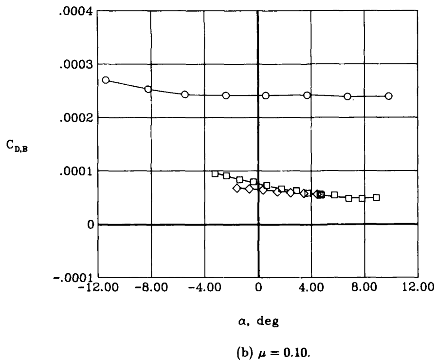
Figure 26. Effect of horizontal tail on airframe drag characteristics. MMS off.
