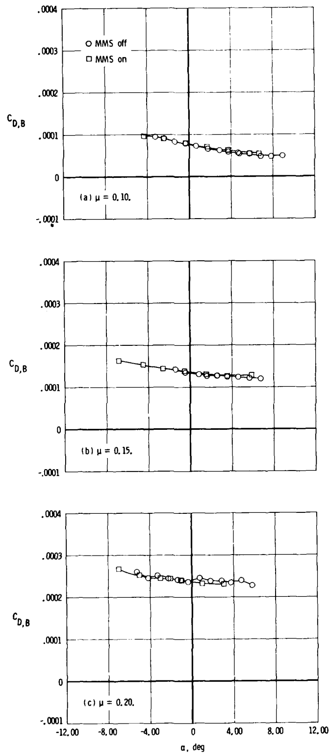
Figure 31. Effect of MMS on airframe drag with rotor on.
