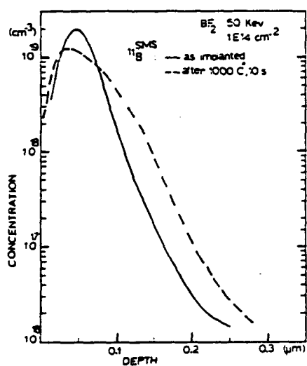
Fig. 4: Boron concentration as a function of depth before and after RTA.
