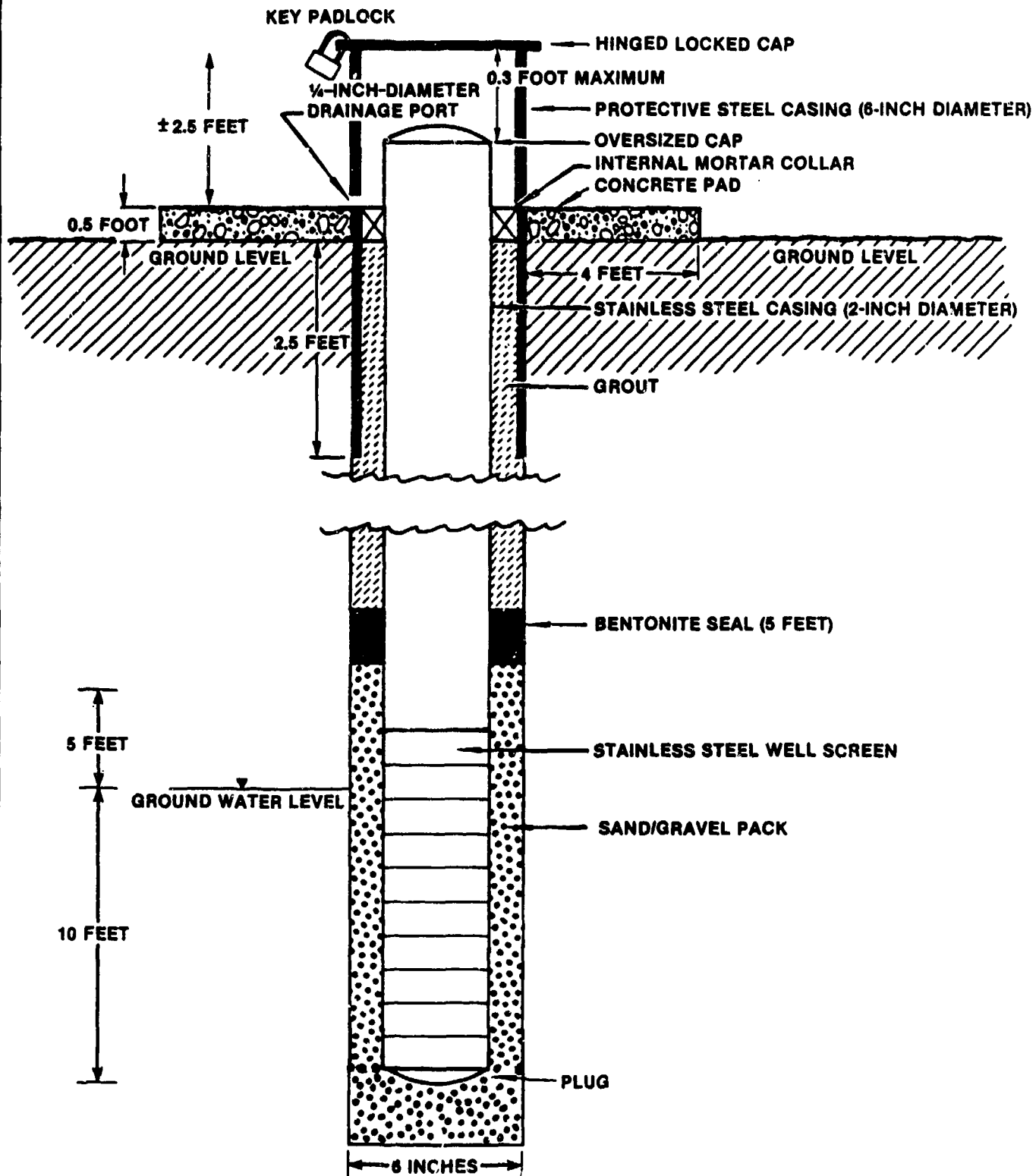
Figure 6.1-2 RECOMMENDED MONITOR WELL CONSTRUCTION DETAILS
