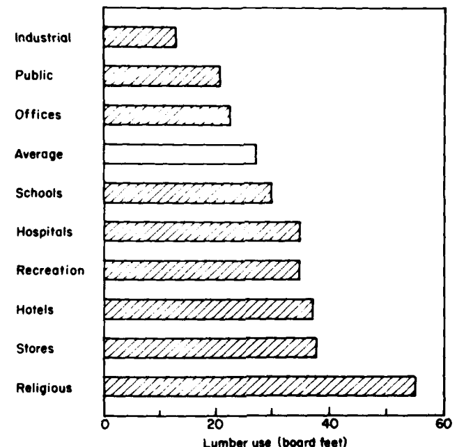
Figure 7.—Lumber use per 1,000 1982 dollars, by building type. (ML84 5629)
