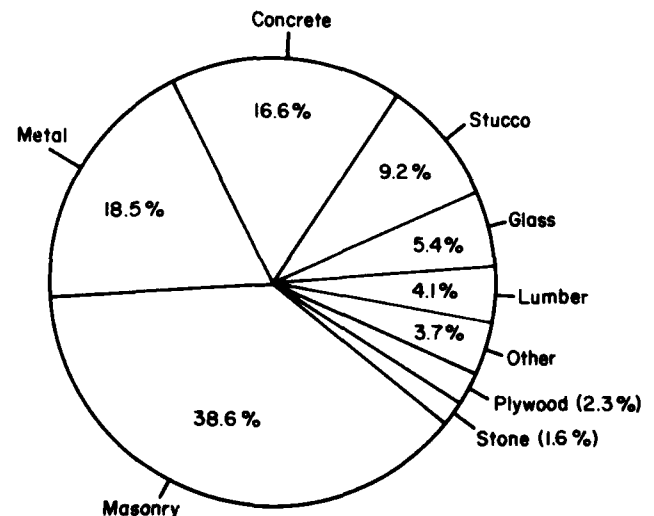
Figure 11.—Percentages of materials used for exterior siding, by area of exterior walls. (ML84 5633)
