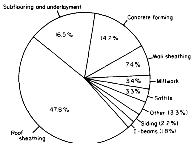
Figure 5.—Plywood used in nonresidential construction by building component, 1982. Total 1.7 billion square feet (3/8-in. basis). (ML84 5637)
