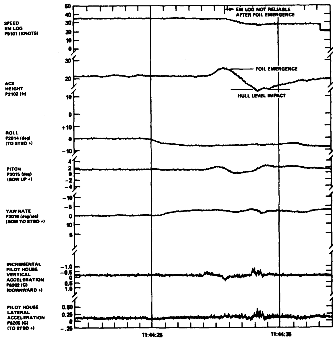
Figure 30 - Data Traces--Broach-in-Turn at 36 Knots, 60° Port Helm
