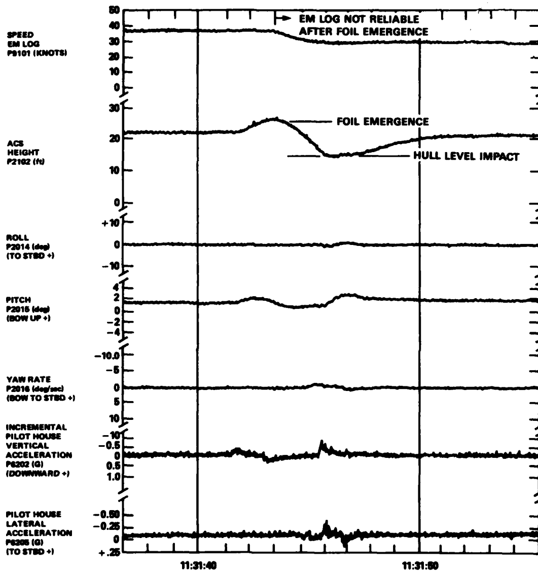
Figure 27 - Data Traces--Straightaway Broach at 36 Knots, 0° Helm
