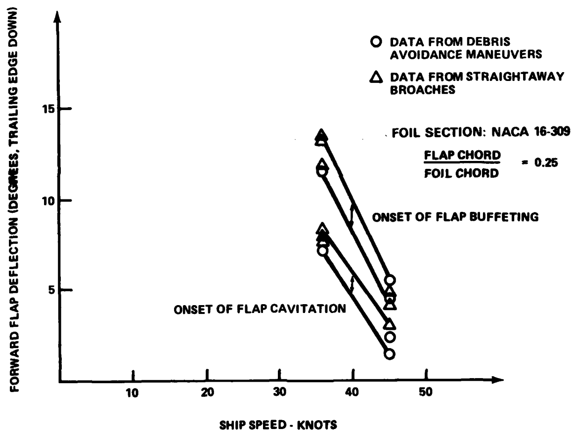
Figure 22 - Forward Flap Deflection for Onset of Cavitation and Buffeting versus Ship's Speed
