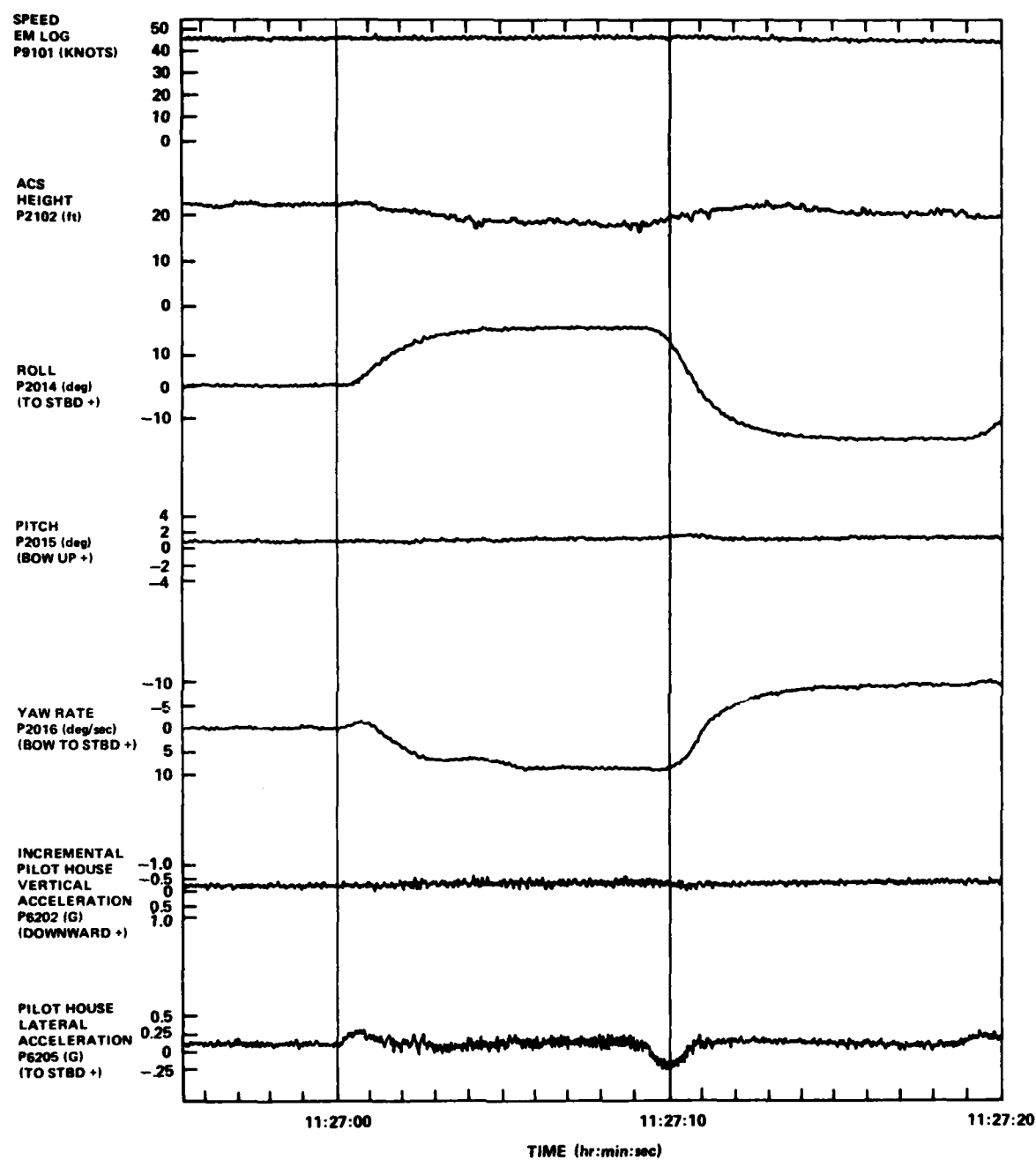
Figure 5 - Data Traces--Debris Avoidance Maneuver at 45 Knots with 180° Helm Displacement
