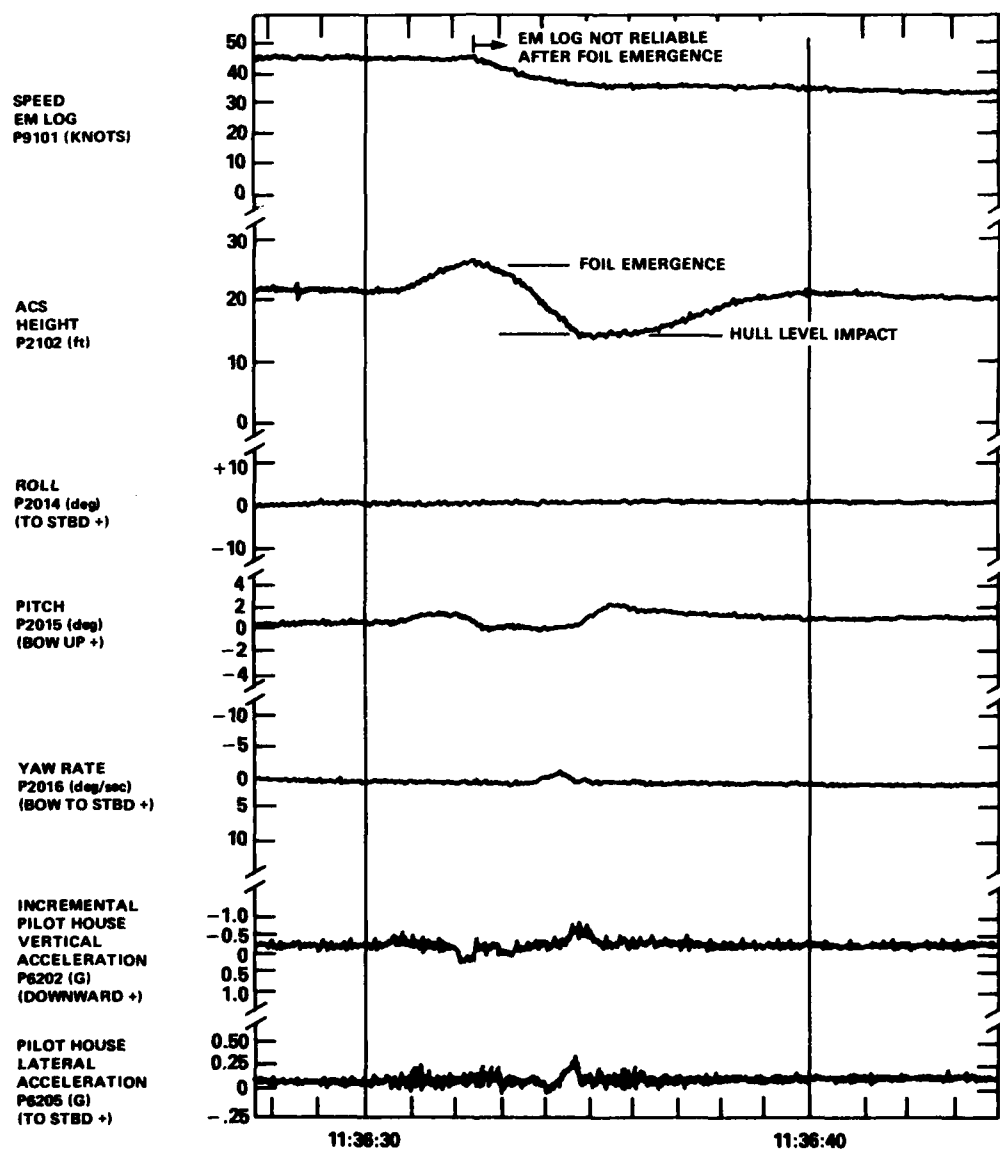
Figure 28 - Data Traces--Straightaway Broach at 45 Knots, 0° Helm
