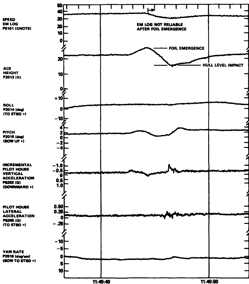
Figure 29 - Data Traces--Broech-in-Turn at 36 Knots, 30° Starboard Helm
