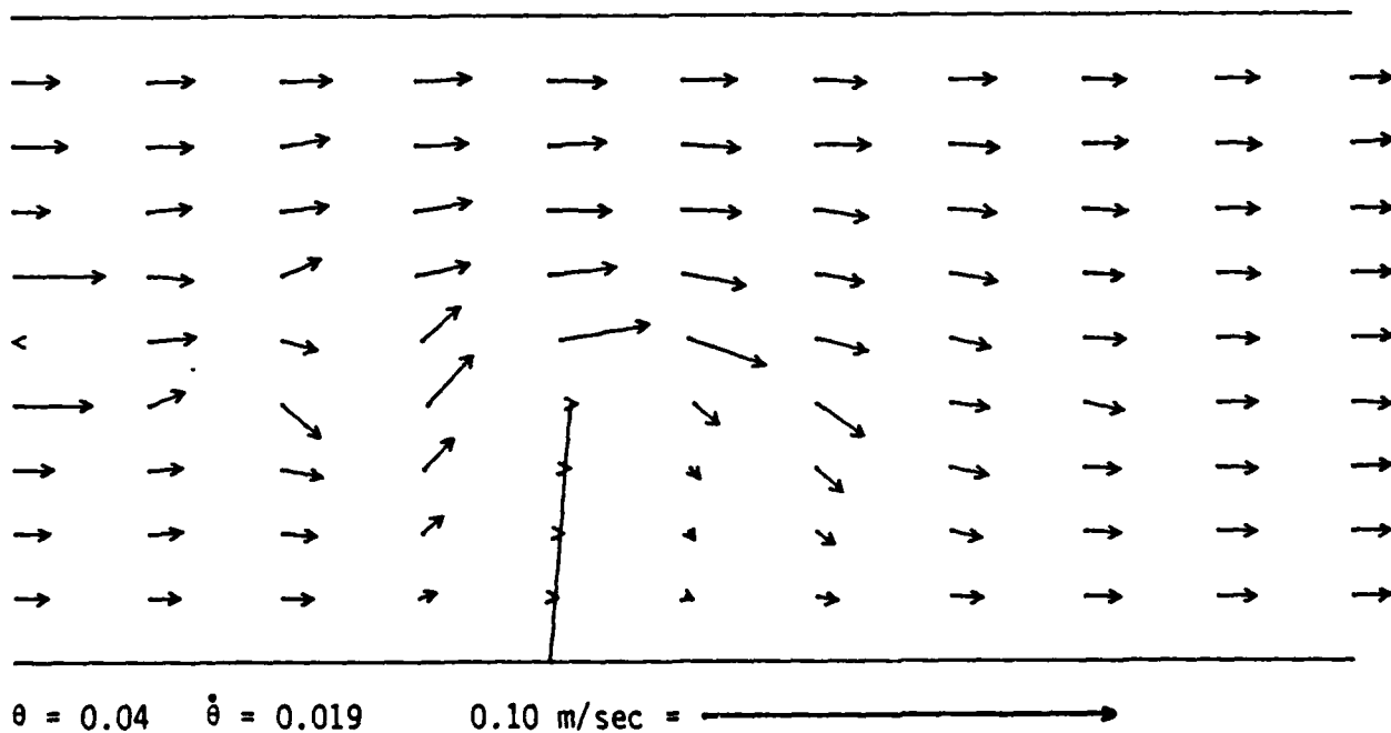
FIGURE 3. Interactive flap velocity field, inlet v = 0
