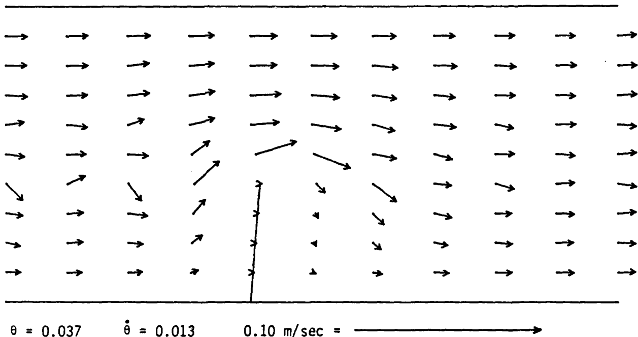
FIGURE 2. Interactive flap velocity field, inlet \beta_v = 0
