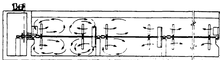
Axial-flow propeller flocculator. This mixing unit is similar to the paddle reel flocculator.
