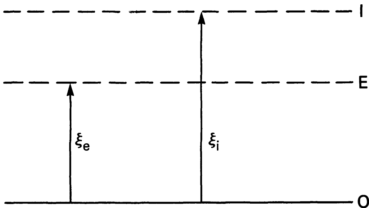
Fig. 1 — Electron sheet E and ion sheet I displaced from their equilibrium position 0.
