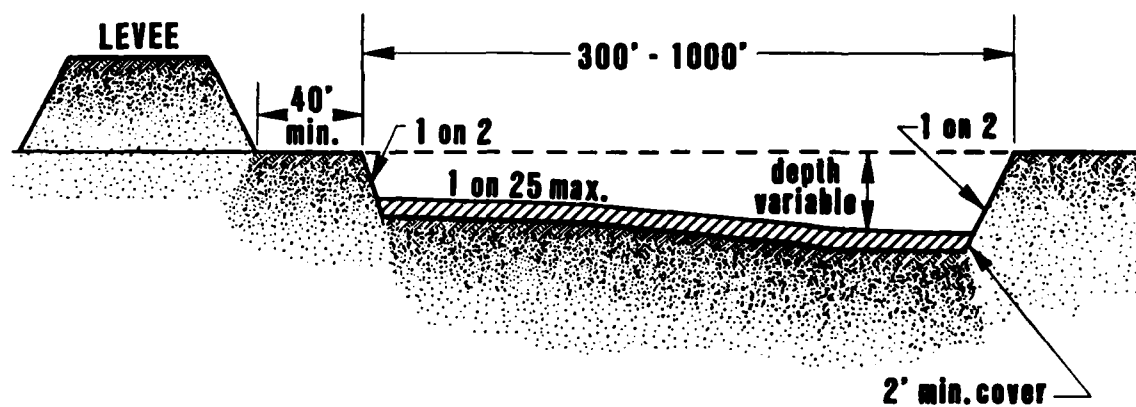
Figure 2. Cross section of a typical Lower Mississippi River main stem levee and borrow area. The 2-foot minimum cover is a layer or cap of relatively impervious soil left in the bottom of the borrow pit to retard underseepage.
