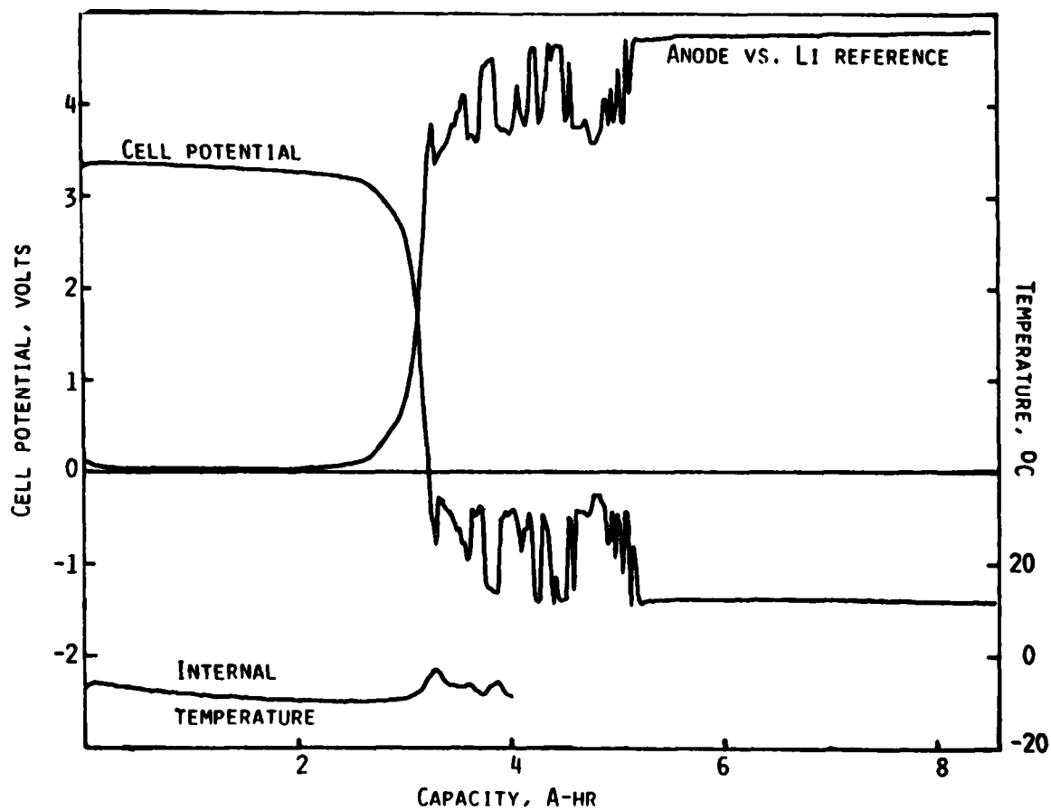
FIGURE 6. DISCHARGE DATA FOR CELL C-A-D-10 AT 0.2A AND -12°C
