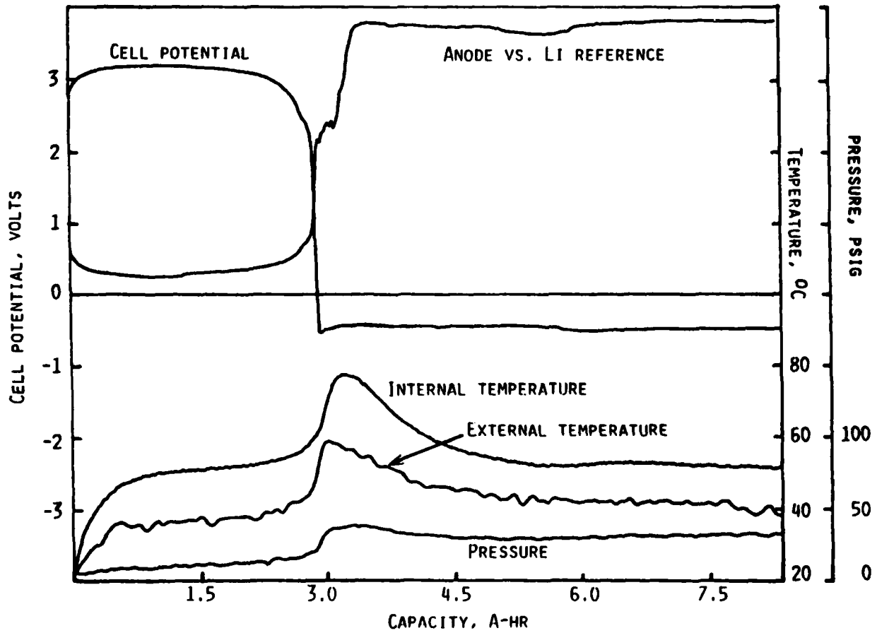
FIGURE 3. DISCHARGE DATA FOR CELL C-A-D-7 AT 3.0A AND 20°C
