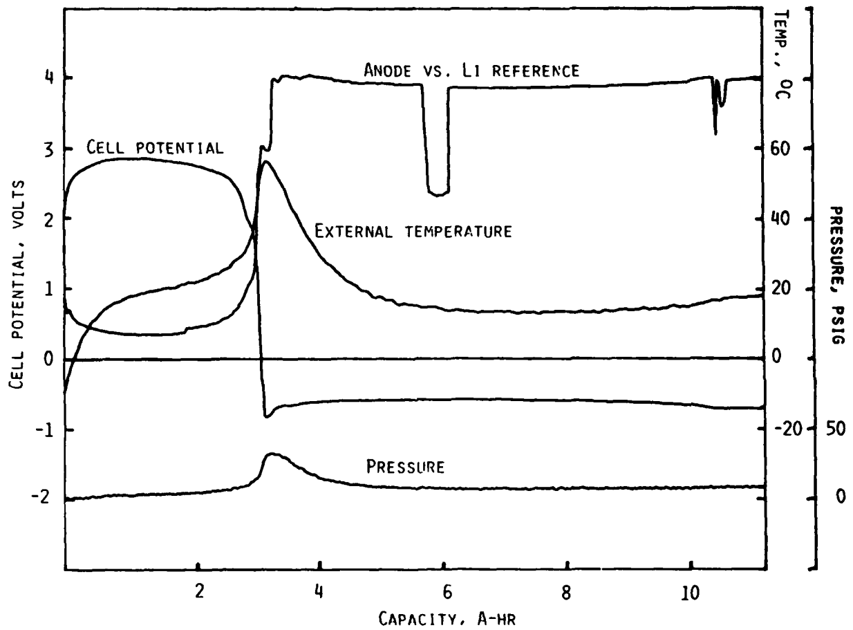
FIGURE 10. DISCHARGE DATA FOR CELL C-A-W-26 AT 4.0A AND -12°C
