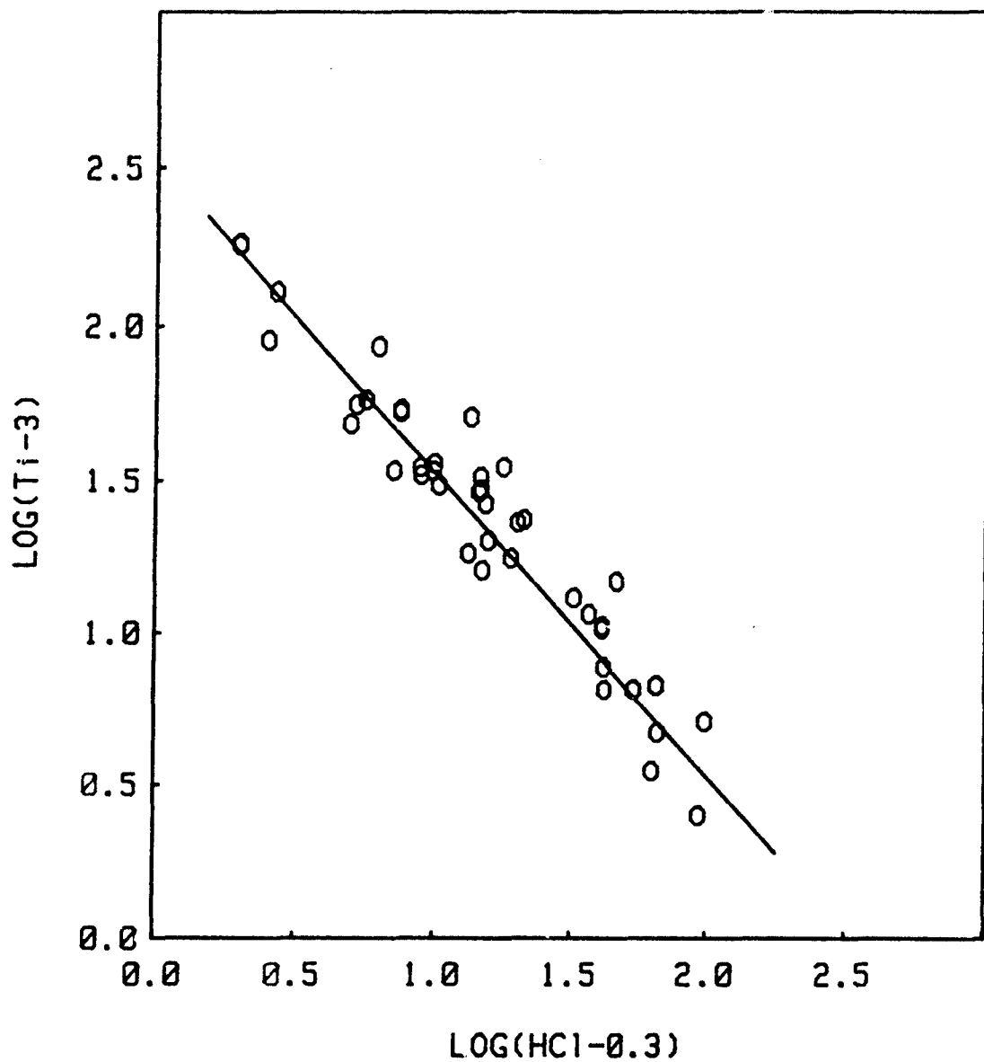
Figure 5. Log-log plot of (t_i-3) versus (HCl-0.3) , a linearized form of the equation relating response time to concentration. (N=43, time is in minutes, concentration is in parts per thousand, regression correlation coefficient=0.96.)
