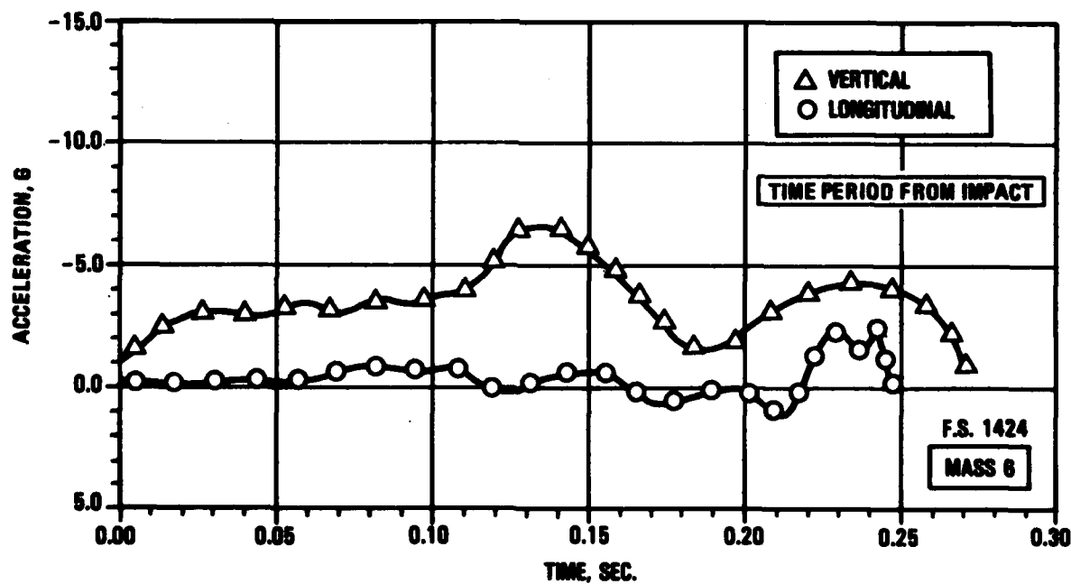
Figure 5-17. - Airframe responses, air-to-ground hard landings, AGHL-358-2. 4
