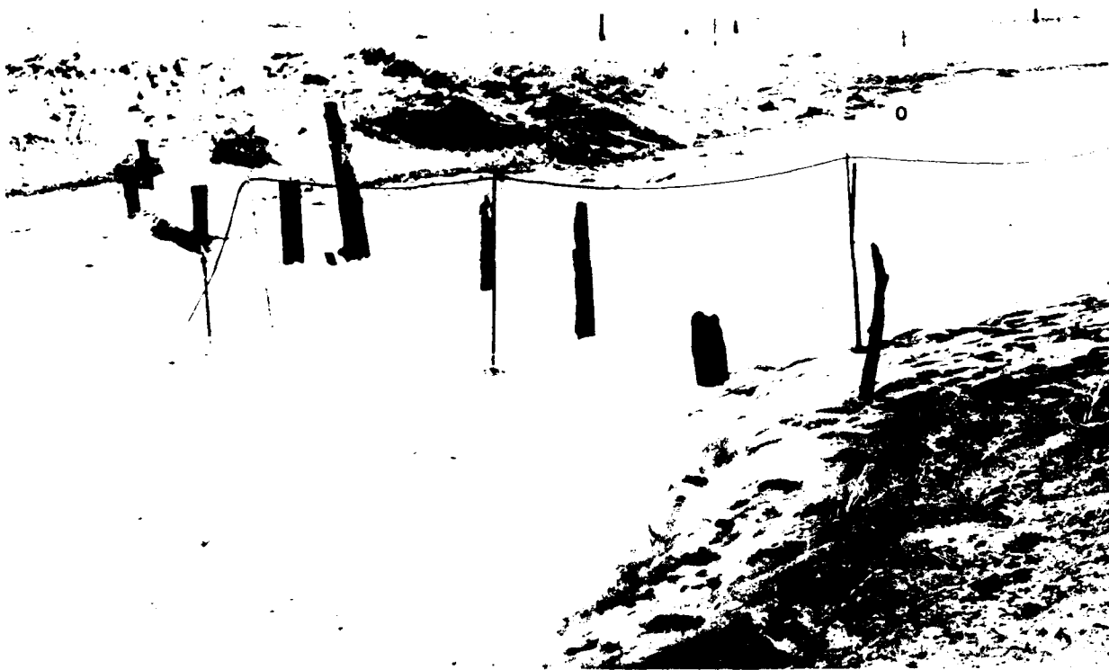
Figure 7. Frontal bore of overwash surge passing the flow sensors.
