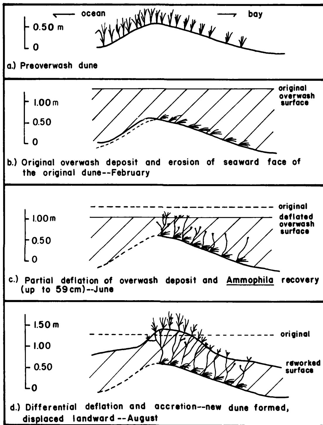
Figure 45. Model of direct overwash involvement in dune building.
