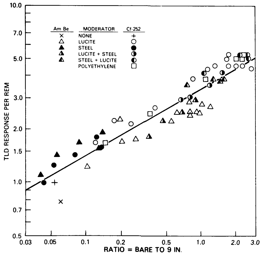
Fig. 5 — The neutron response per Rem of the ^6\text{LiF} detector behind the cadmium shield vs the bare to 9-in. detector ratio
