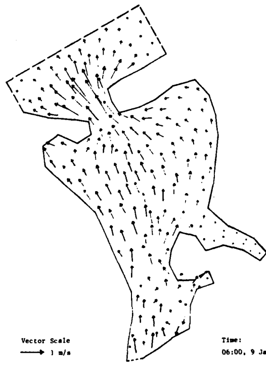
b. Ebb tide at Bechevin Inlet
