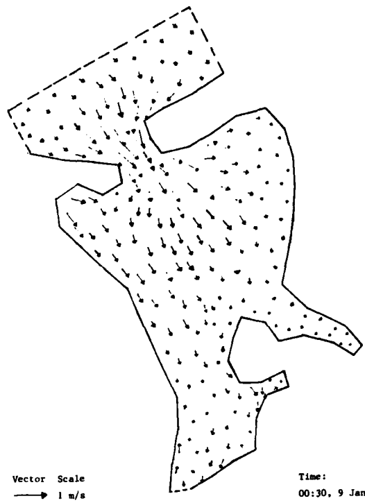
a. Flood tide at Bechevin Inlet
