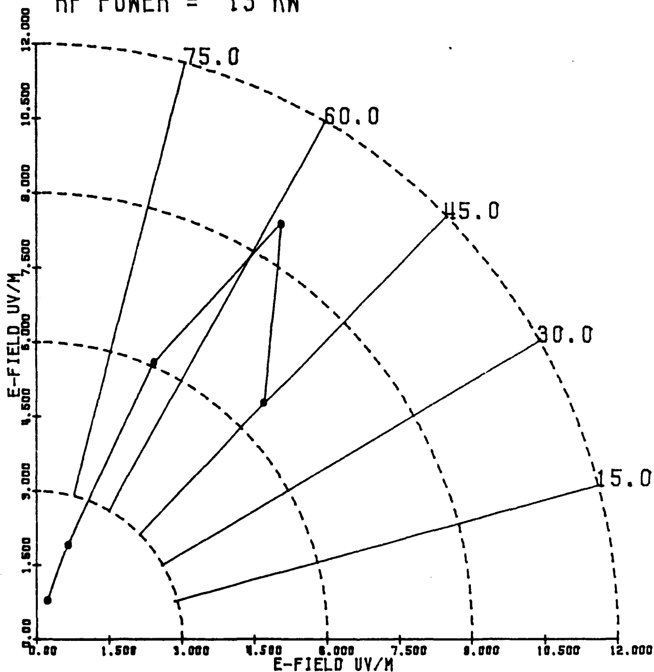
FIGURE 8. MACHINE B CLARK TOWER DATA NORMALIZED TO 1000 FEET AT 0° AZIMUTH DECAY FACTOR = 2.45.
