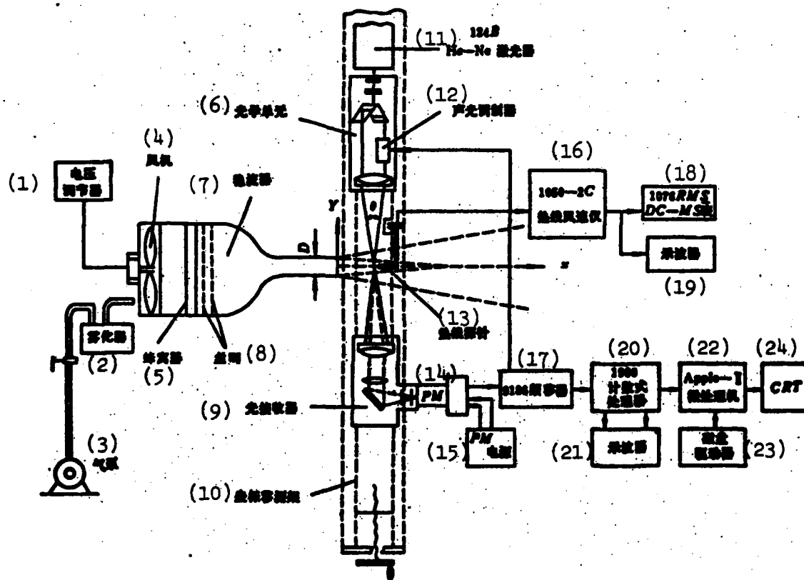
Fig. 1 Schematic diagram of the experimental apparatuses and measurement systems.
