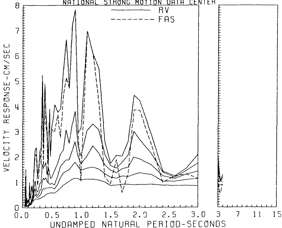
Figure 6b. Velocity response spectrum and Fourier amplitude spectrum at Upper Intake Tower, V-component, at Ririe Dam
