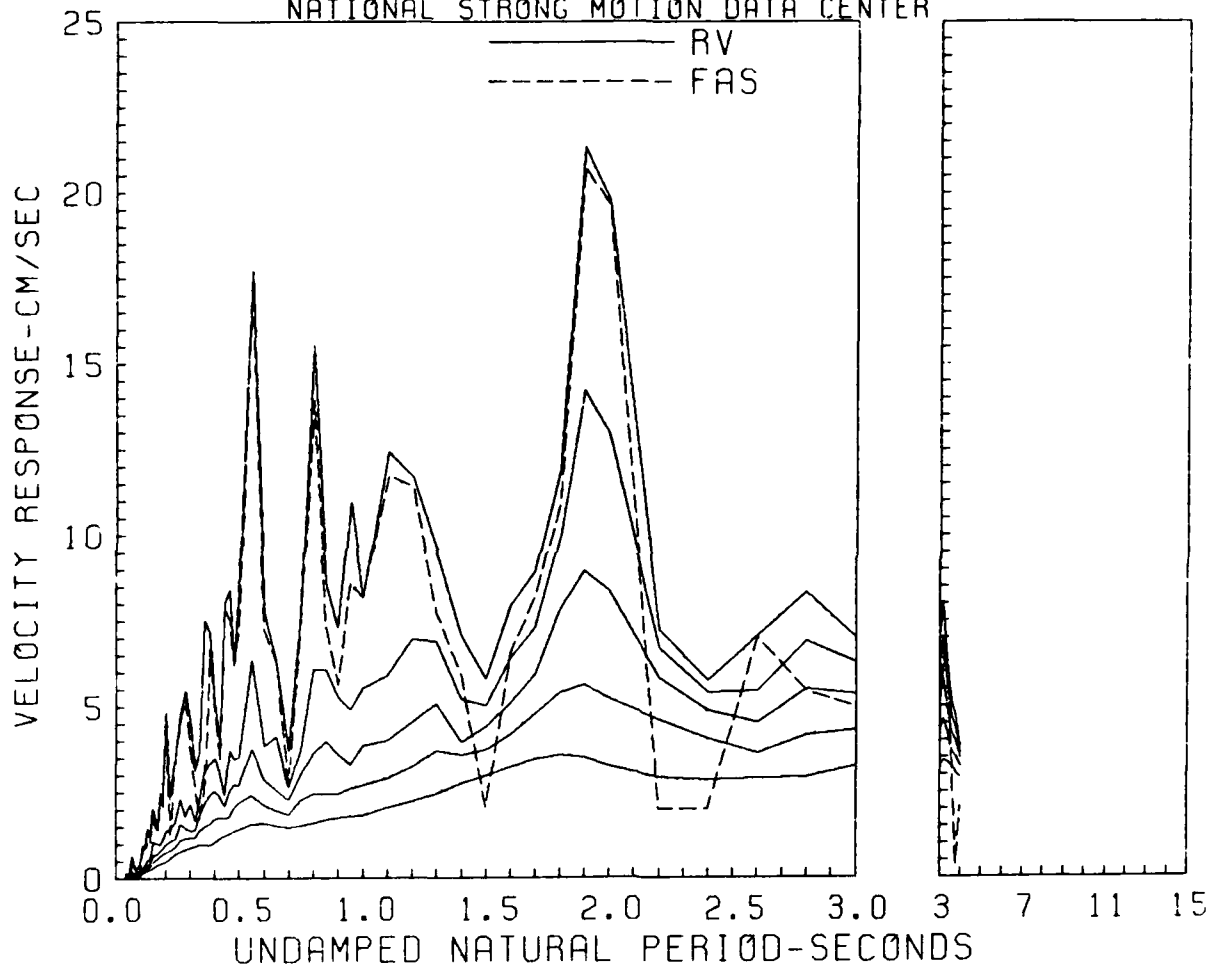
Figure 5a. Velocity response spectrum and Fourier amplitude spectrum at left abutment, L-component, at Ririe Dam
