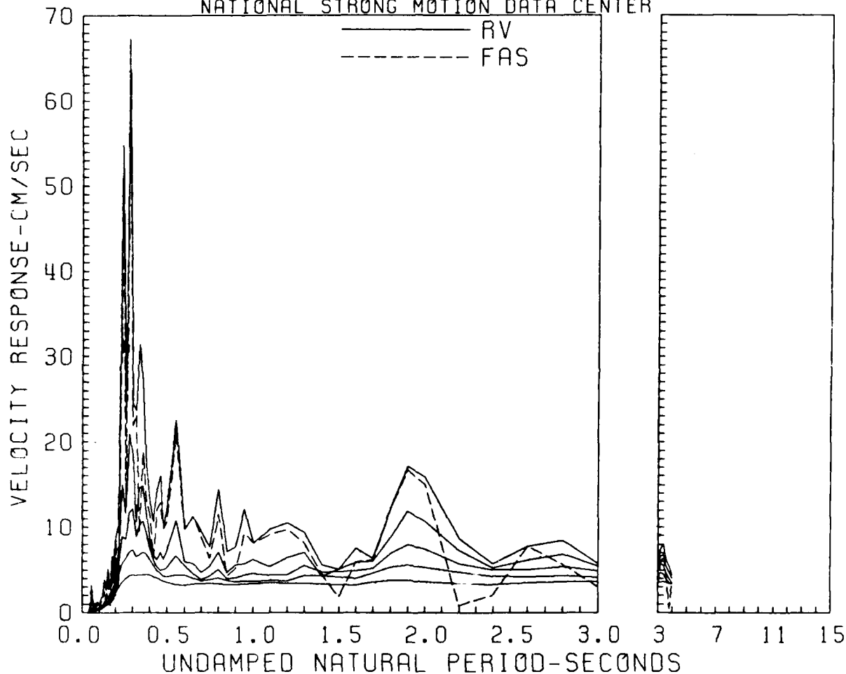
Figure 6a. Velocity response spectrum and Fourier amplitude spectrum at Upper Intake Tower, L-component, at Ririe Dam
