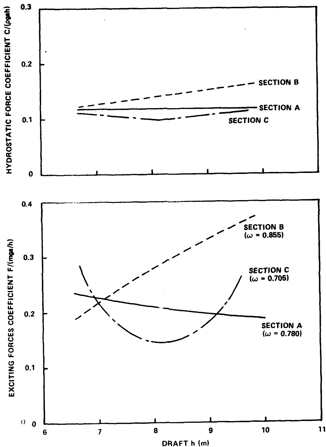
Figure 4 - Hydrostatic and Exciting Forces Coefficients of SWATH Sections for Heave Resonance as a Function of Draft
