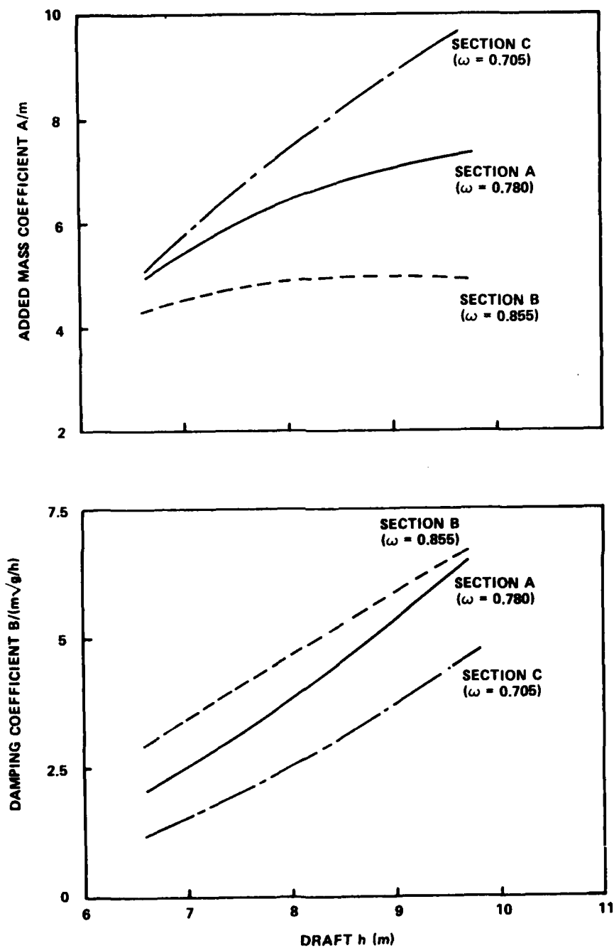
Figure 5 - Added Mass and Damping Coefficients of SWATH Sections for Heave Resonance as a Function of Draft
