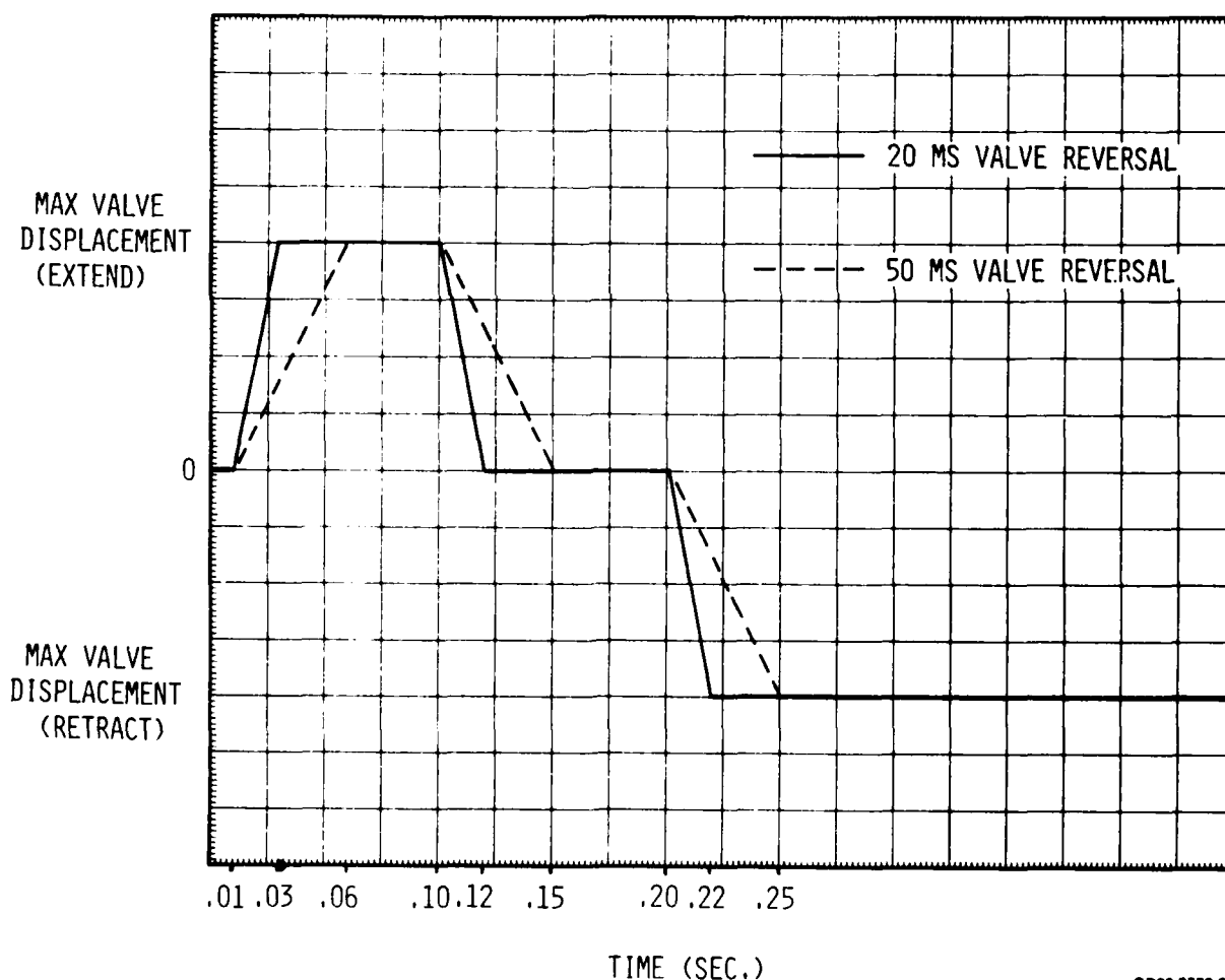
Figure 130. F-15 SPEEDBRAKE OPERATING CYCLE
