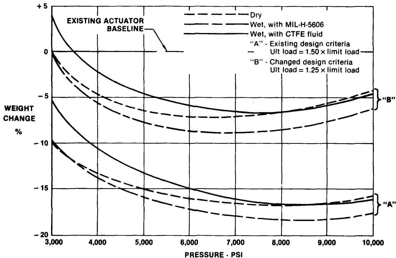
Figure 83. INBOARD ELEVATOR ACTUATOR ASSEMBLY WEIGHT CHANGE With Aluminum Manifolds Ult Load = 1.25 x Limit Load
