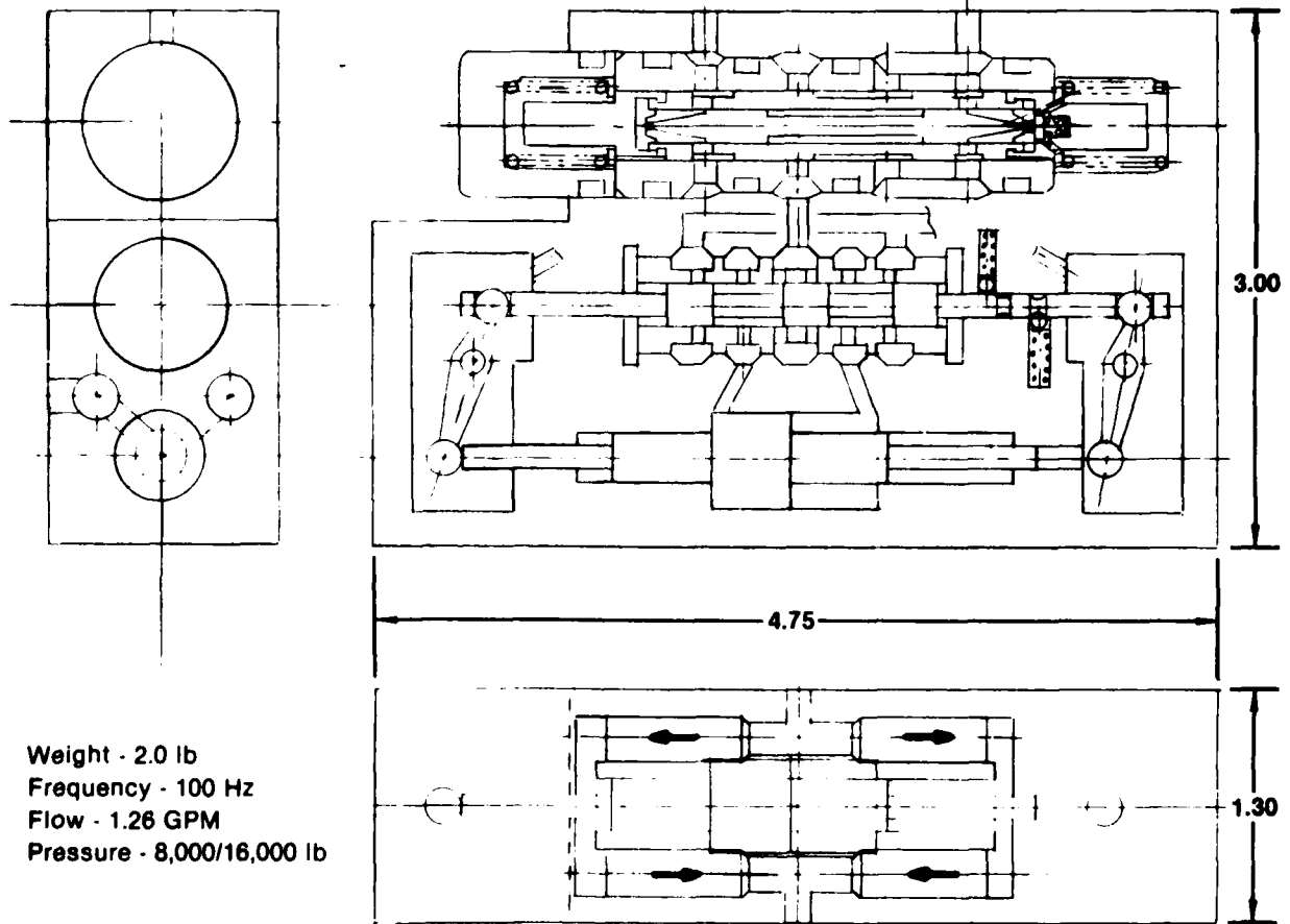
Figure 224. MCAIR PRESSURE INTENSIFIER
