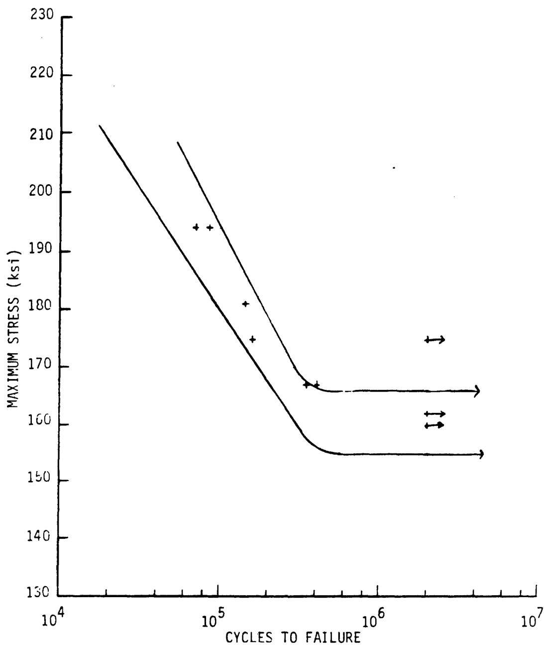
Figure 5-8. The S-N Curves of As Received and Reheat Treated Tank Track Pin T-142 Along With Data Points from Fatigue Testing of Recycled Pins Shown as '+'.
