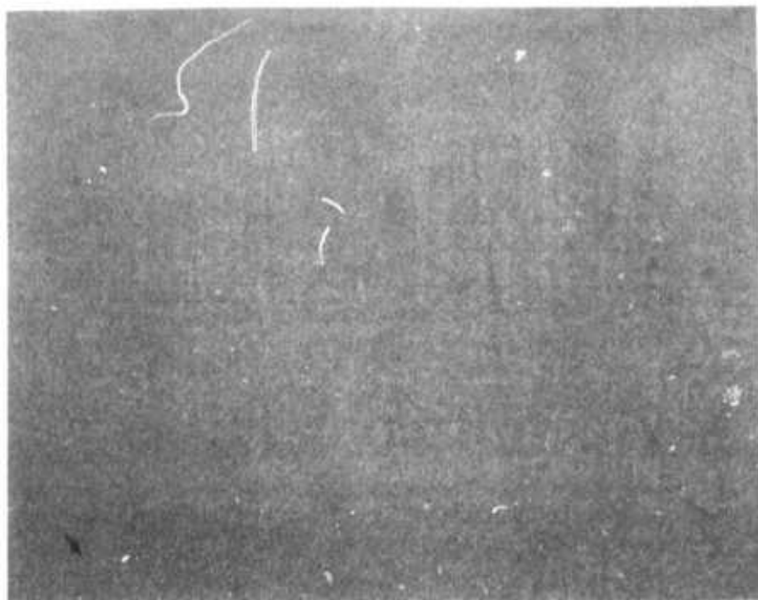
Fig. 12 Surface of \text{CaF}_2 Sample After Optical Polish (Pitch Lap). 187\times
