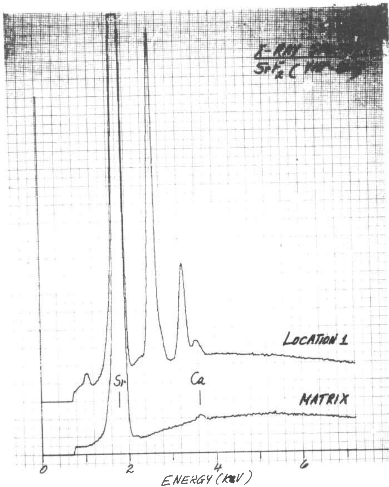
Fig. 5a X-Ray Spectra of Cast \text{SrF}_2 Sample
