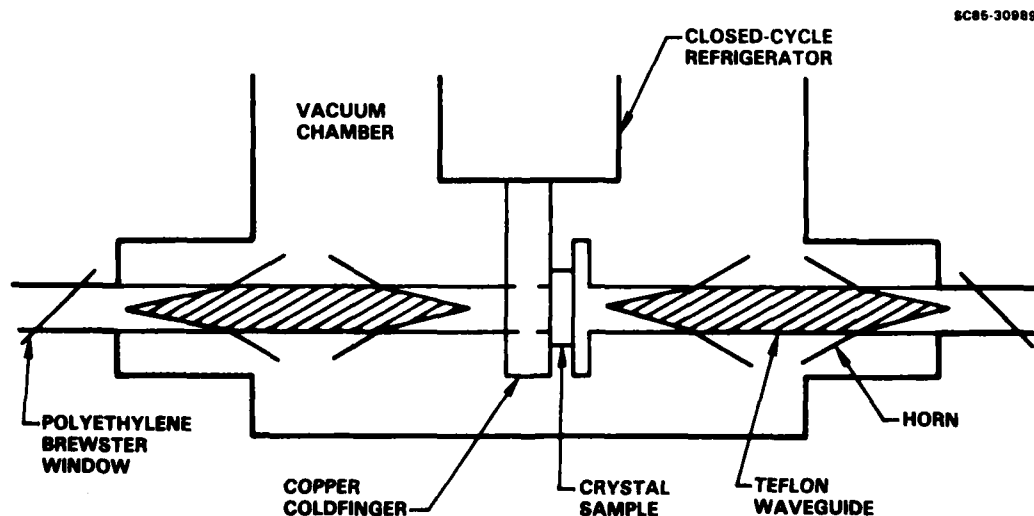
Fig. 4 Millimeter wave transmittance measurement apparatus (UCLA).
