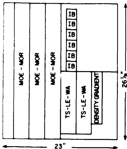
Figure 3—Cutup diagram for 1-1 4- and 2-inch-thick boards. Sample size: same as figure 2 except modulus of elasticity (MOE) and modulus of rupture (MOR) 3 by 26 inches. (ML83 5072)
