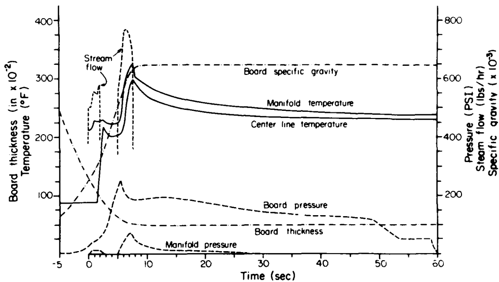
Figure 7—A brief exposure to maximum temperatures of 325 °F permits resin cure at 235 °F in 60 seconds press time, 1 2-inch-thick 0.640 SG board (5.24d). (ML85 5076)
