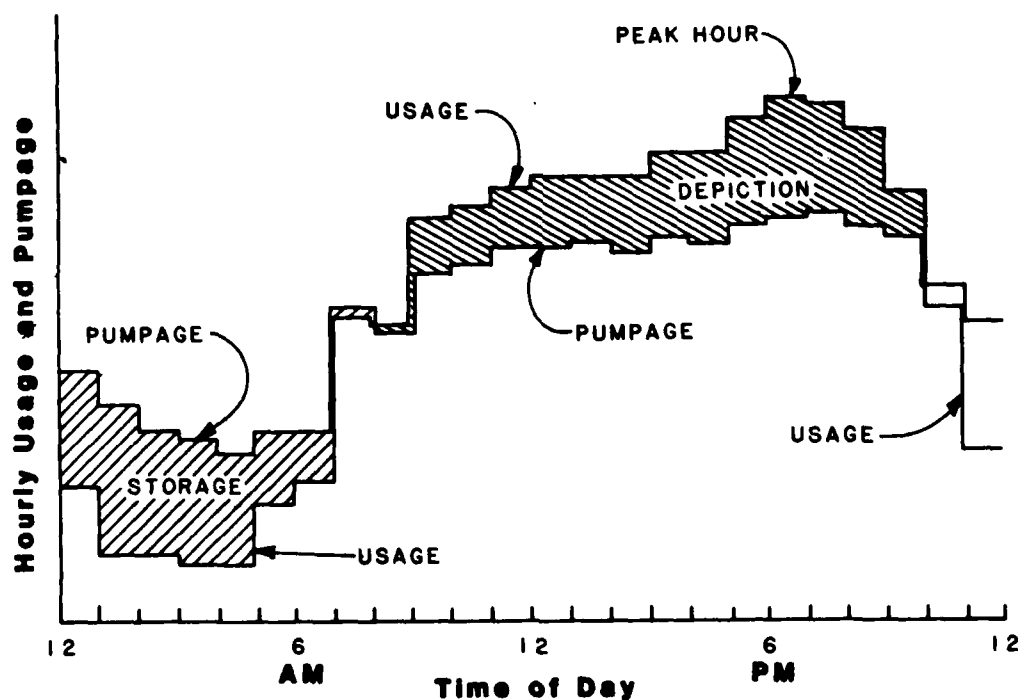
Figure 2. Analysis of Maximum Day Usage of Madison, Wisconsin, Water Utility
