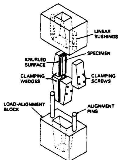
Figure 13. IITRI Compression Test Fixture Using Pyramidal Wedges
