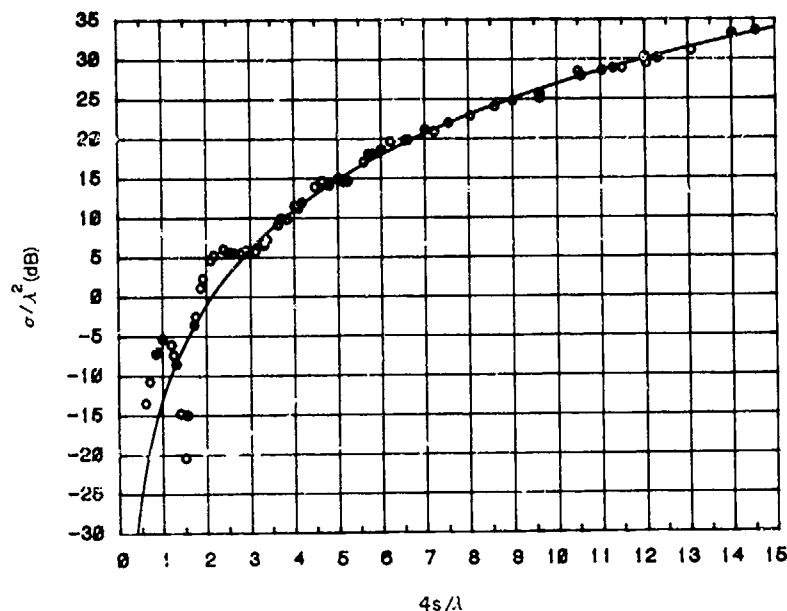
Figure 6. Cube RCS Measurements Compared With Physical Optics Solution. Theory —, Measured o
