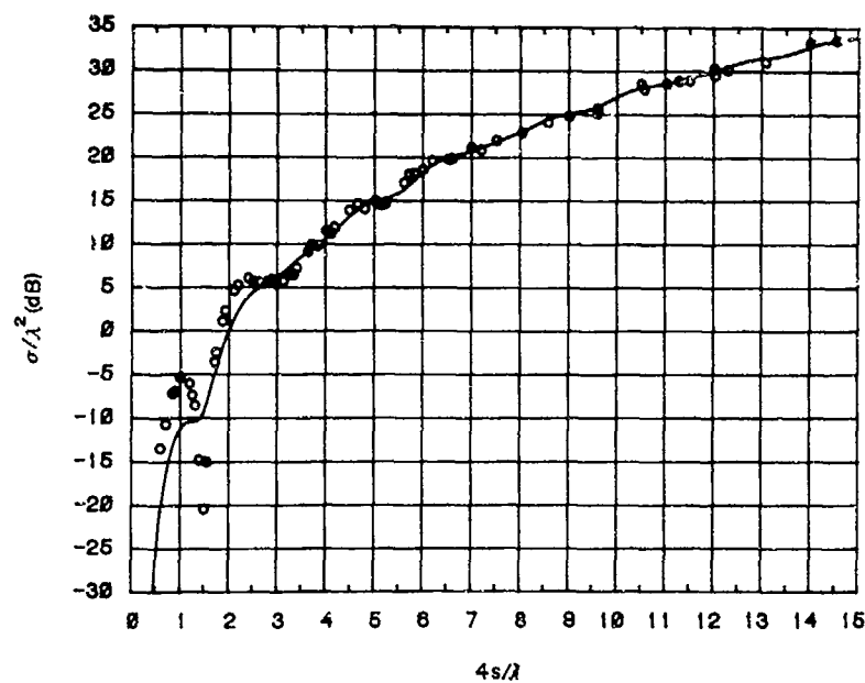
Figure 7. Cube RCS Measurements Compared With High Frequency Diffraction Solution. Theory —, Measured \circ
