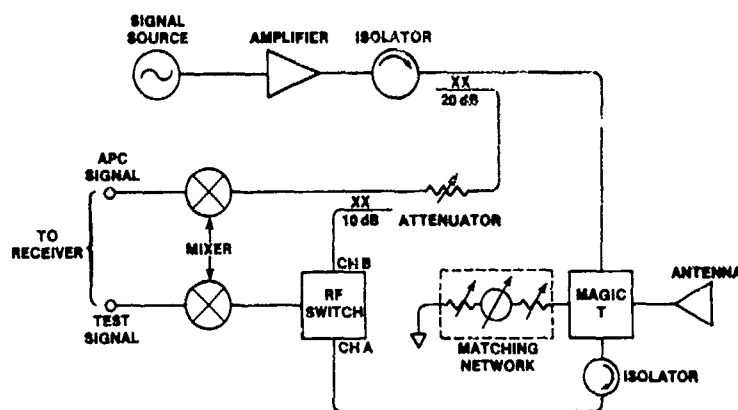
Figure 5. Measurement System for Cube RCS Measurements
