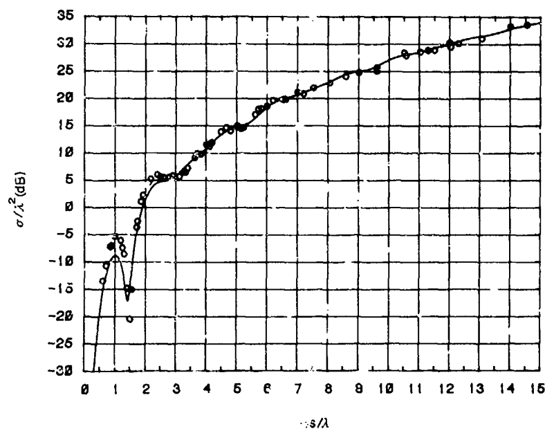
Figure 8. Cube RCS Measurements Compared With Enhanced High Frequency Diffraction Solution. Theory —, Measured \circ
