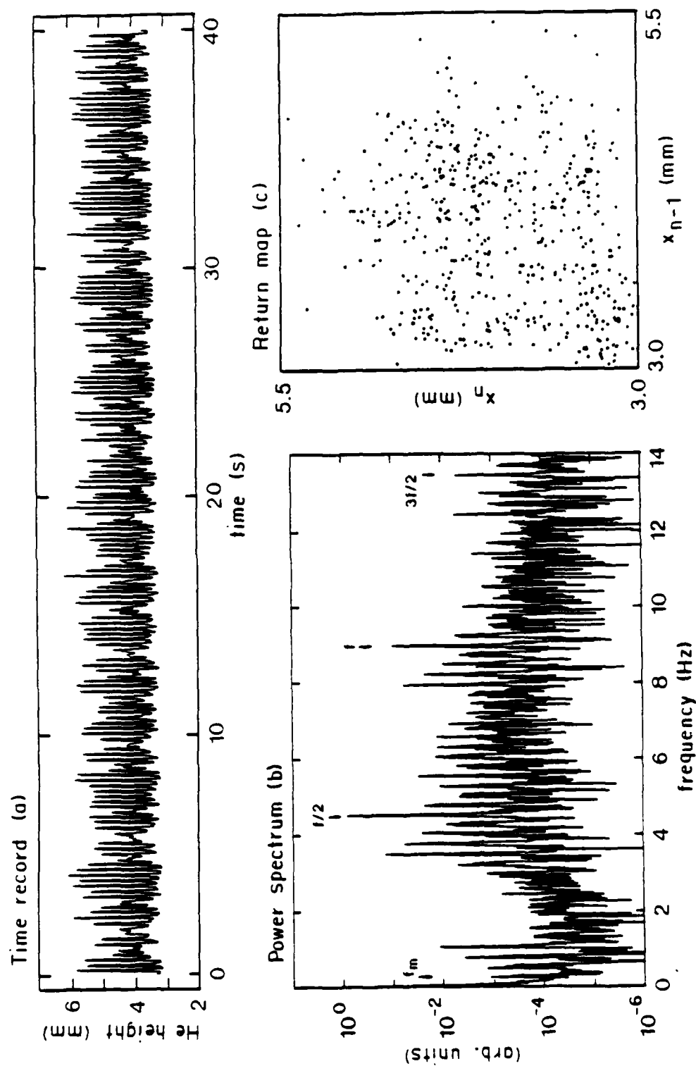
Figure 56. At least three modulations out of lock, with 29.1 \mu\text{m} rms drive amplitude.
