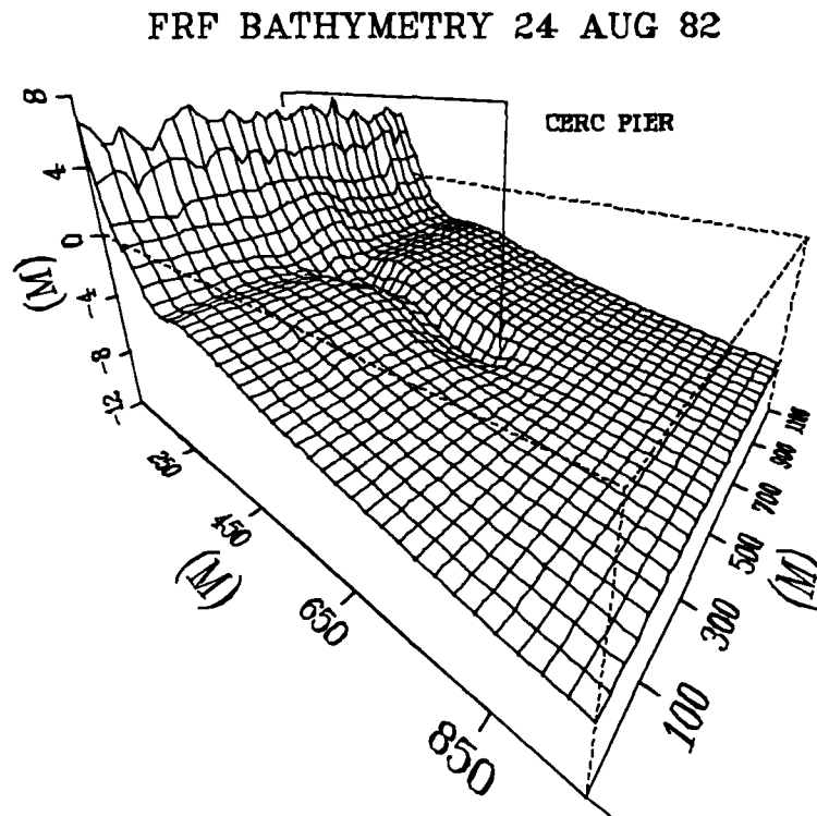
Figure 30. FRF bathymetry, 24 August 1982
