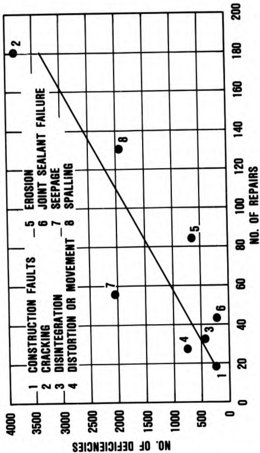
Figure 20. Relationship between number of observed deficiencies and number repaired for eight general categories of observed deficiencies
