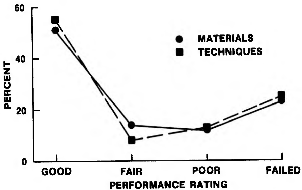
Figure 23. Relative performance of repair materials and techniques
