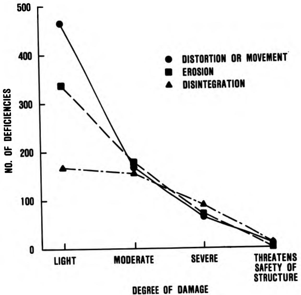
Figure 9. Relationship between number of distortion or movement, erosion, and disintegration deficiencies observed and their degree of damage
