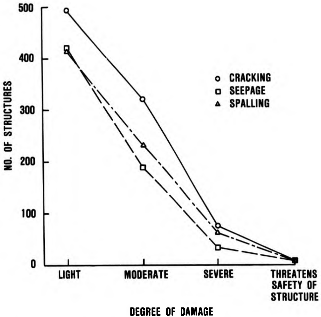
Figure 8. Relationship between number of structures with cracking, seepage, and spalling deficiencies and their degree of damage
