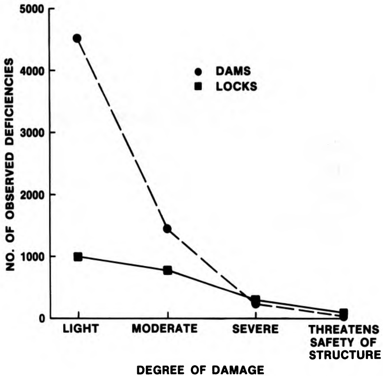
Figure 15. Relationship between number of deficiencies observed in locks and in dams and their degree of damage
