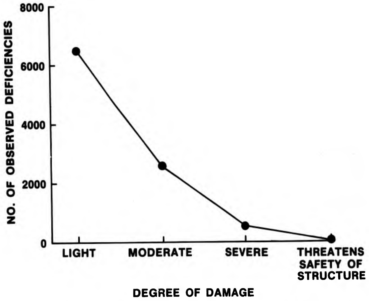
Figure 17. Relationship between number of observed deficiencies and their degree of damage
