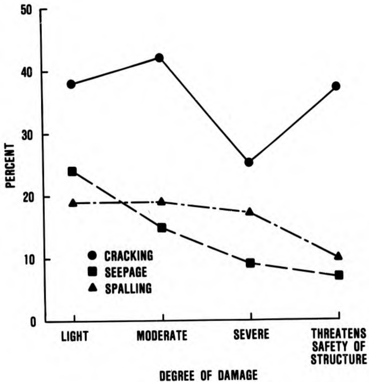
Figure 7. Percentage of total cracking, seepage, and spalling deficiencies within the various degree of damage classifications
