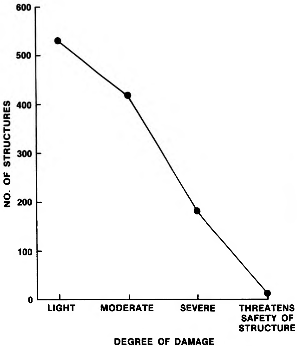
Figure 18. Relationship between number of structures with observed deficiencies and their degree of damage
