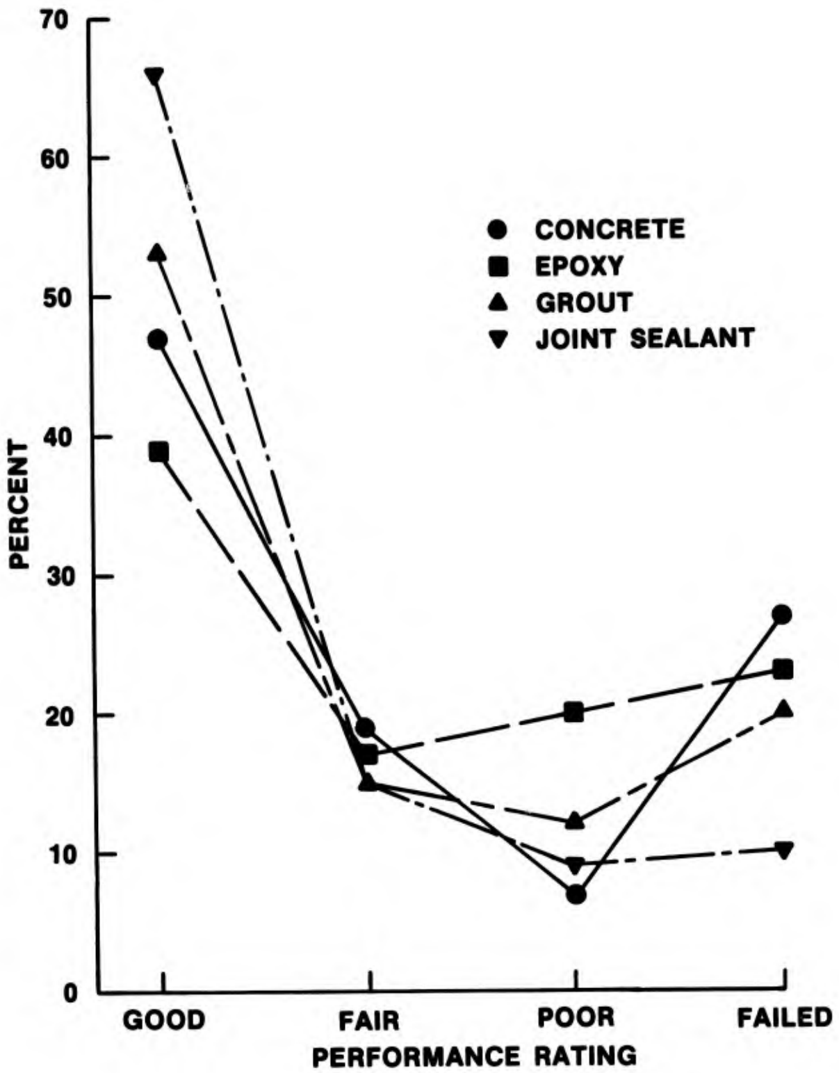
Figure 22. Relative performance of four general types of repair materials
