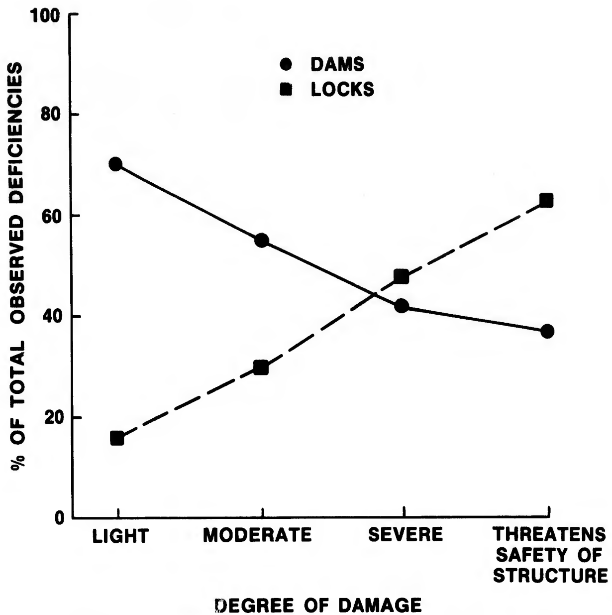
Figure 16. Relationship between percentage of total observed deficiencies in locks and in dams and their degree of damage
