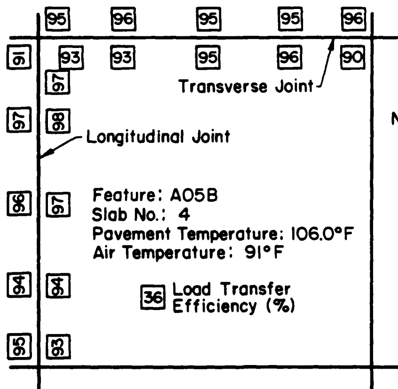
Figure 4-9. Joint Load Transfer Efficiencies at Various Locations for Feature A05B, Slab No. 4
