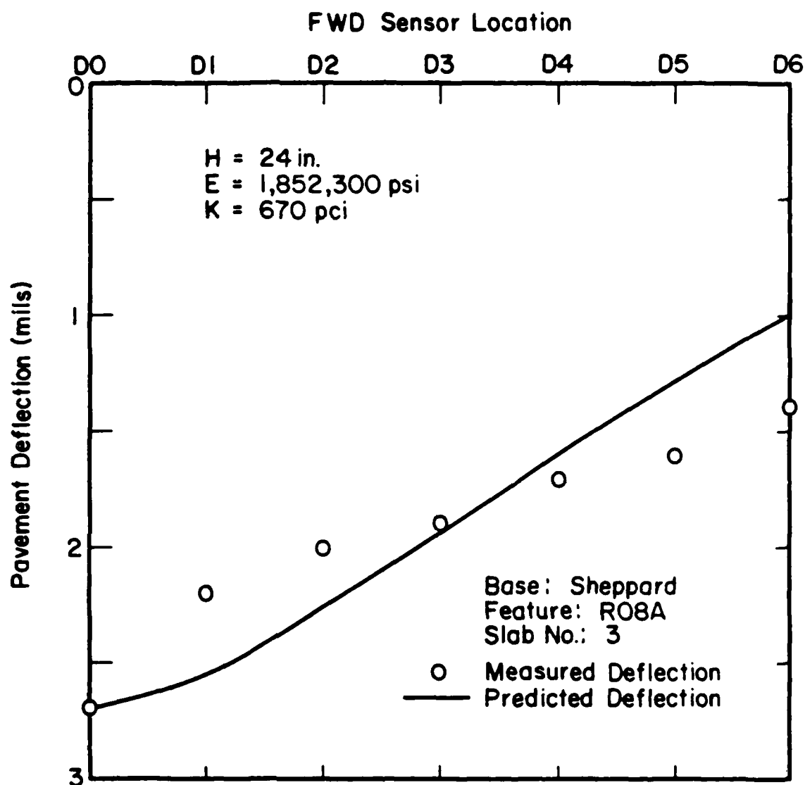
Figure 5-14. Comparison of Measured and Predicted FWD Deflections for Feature R08A
