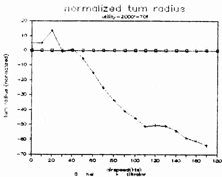
Figure N-V-189. Utility normalized turn radius: helicopter and tilt rotor, 2,000 ft, 70°F.
