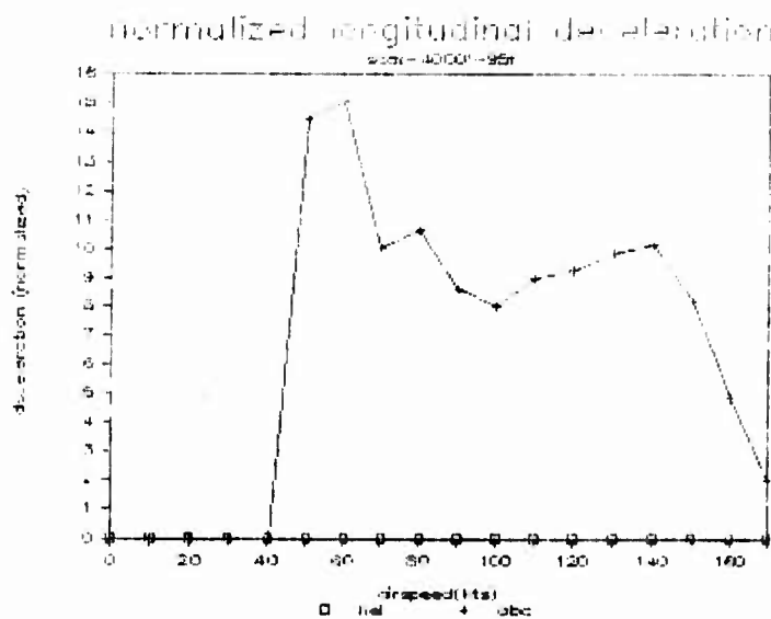
Figure N-V-30. SCAT normalized longitudinal deceleration: helicopter and ABC, 4,000 ft, 95°F.
