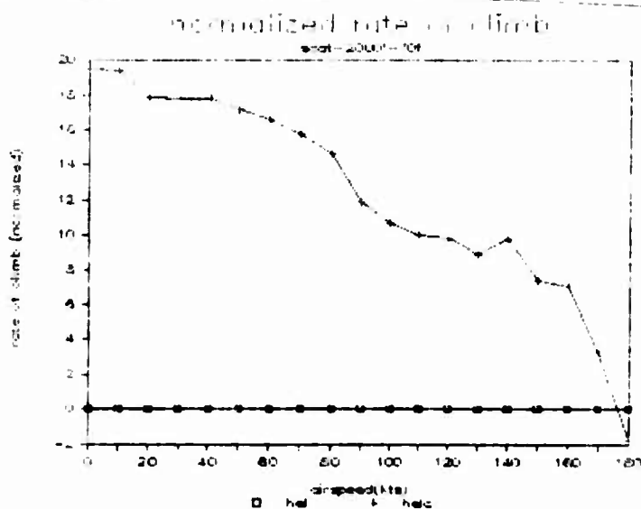
Figure N-V-144. SCAT normalized climb rate: helicopter and helicopter-compound, 2,000 ft, 70°F.
