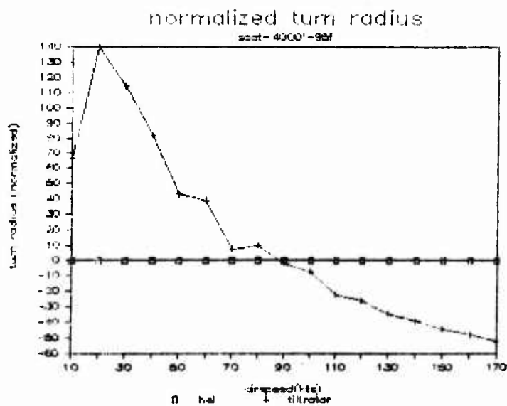
Figure N-V-40. SCAT normalized turn radius: helicopter and tilt rotor, 4,000 ft, 95°F.
