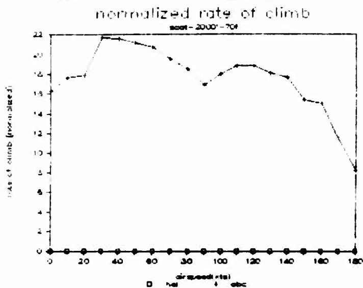
Figure N-V-145. SCAT normalized climb rate: helicopter and ABC, 2,000 ft, 70°F.
