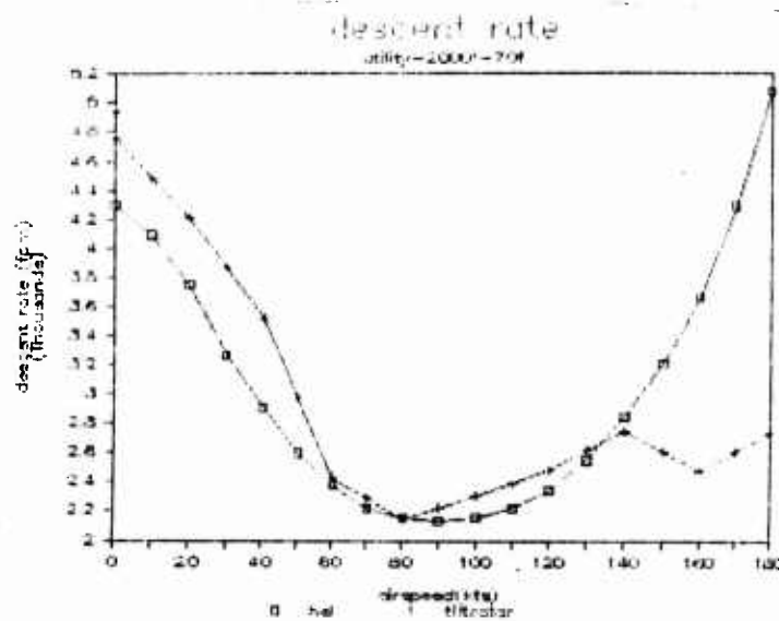
Figure N-V-169. Utility descent rate: helicopter and tilt rotor, 2,000 ft, 70°F.
