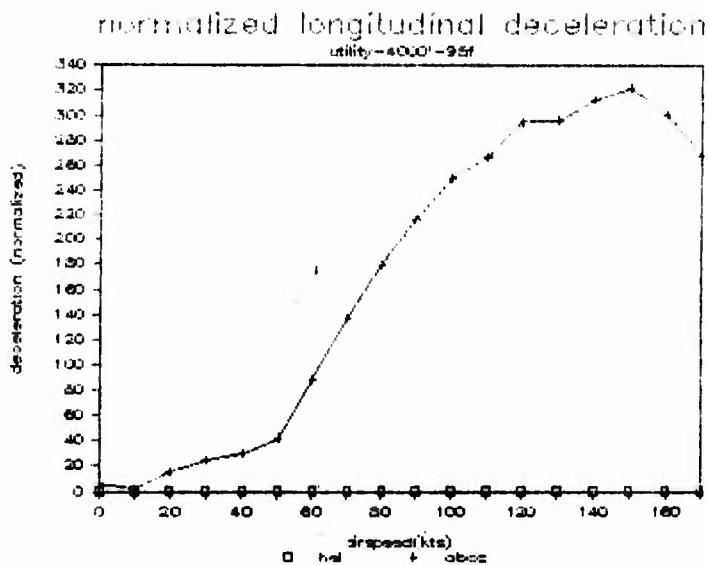
Figure N-V-78. Utility normalized longitudinal deceleration: helicopter and ABC-compound, 4,000 ft, 95°F.
