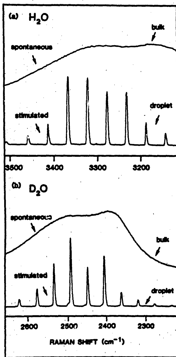
Figure 2. The cw spontaneous Raman scattering from bulk \text{H}_2\text{O} and \text{D}_2\text{O} in a cuvette is shown in the upper spectrum of (a) and (b), respectively. The discrete peaks in the lower spectra of (a) and (b) are from a single droplet using a single 10-nsec laser pulse. These regularly spaced SRS peaks correspond to MDRs.
