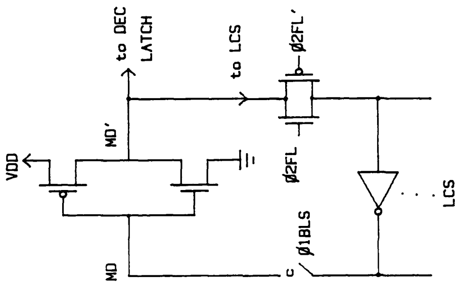
Figure B.3.d.iv. Circuit Schematic of LCS
