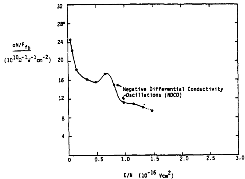
Figure 33. As in Fig. 29, 8:1 He:N 2 (10% CF 4 )/TMA Data
