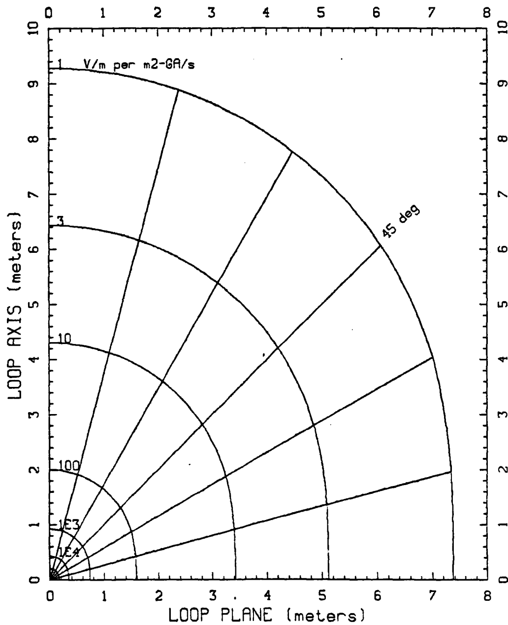
Fig. 58. CLOSE-FIELD PATTERN
