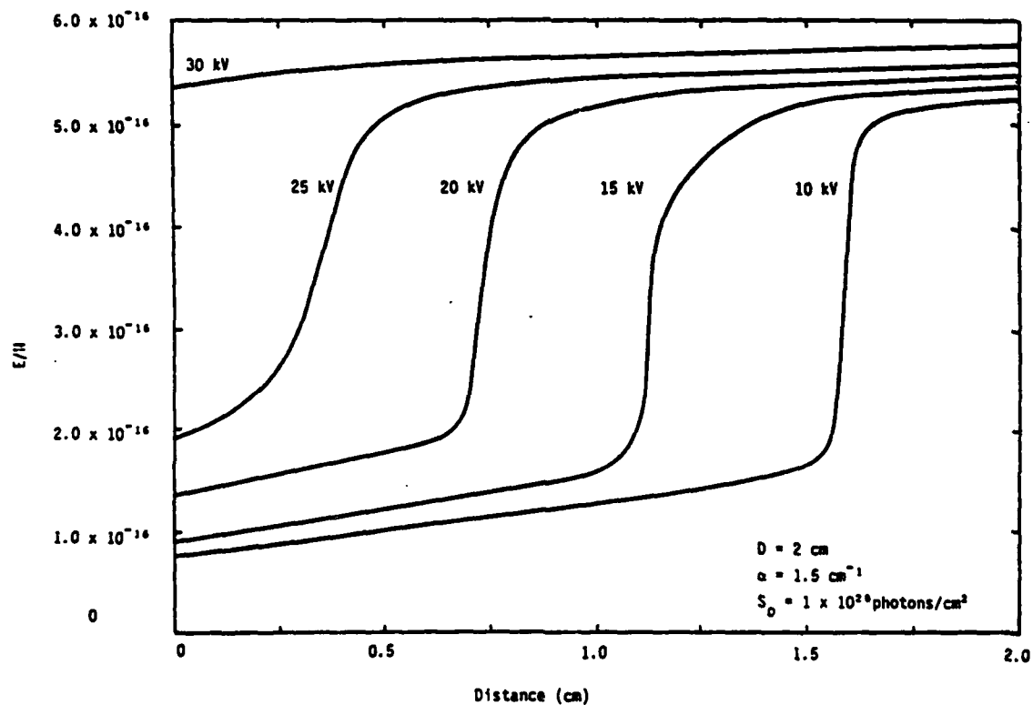
Figure 52 E/N vs Distance
